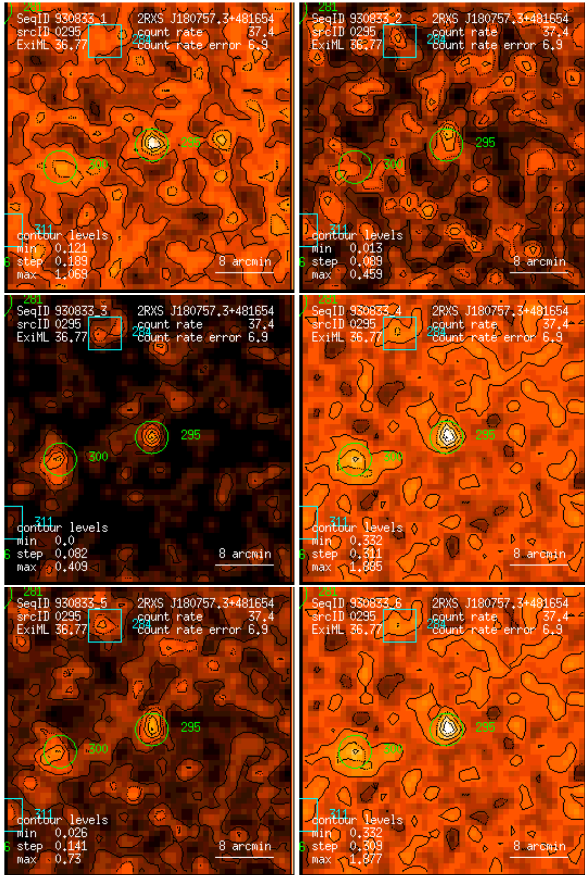
Figure 295: RASS 930833: detection 0295: band rate images, Gaussian filter: (1) PSPC channels 11 – 41, (2) 52 – 90, (3) 91 – 201, (4) 11 – 235, (5) 52 – 201, (6) 11 – 201. Broad band rates in counts/ks. Band rate contour levels in counts/ks/arcmin 2 .
