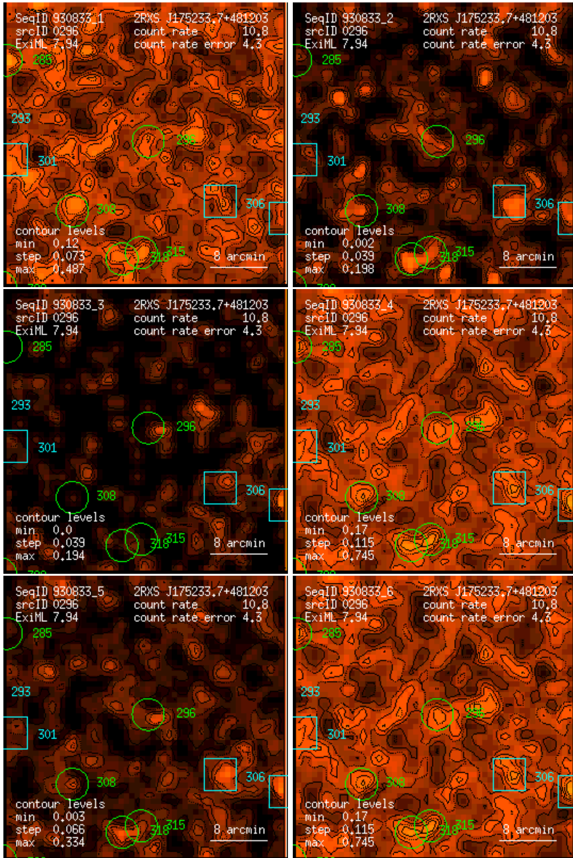
Figure 296: RASS 930833: detection 0296: band rate images, Gaussian filter: (1) PSPC channels 11 – 41, (2) 52 – 90, (3) 91 – 201, (4) 11 – 235, (5) 52 – 201, (6) 11 – 201. Broad band rates in counts/ks. Band rate contour levels in counts/ks/arcmin 2 .
