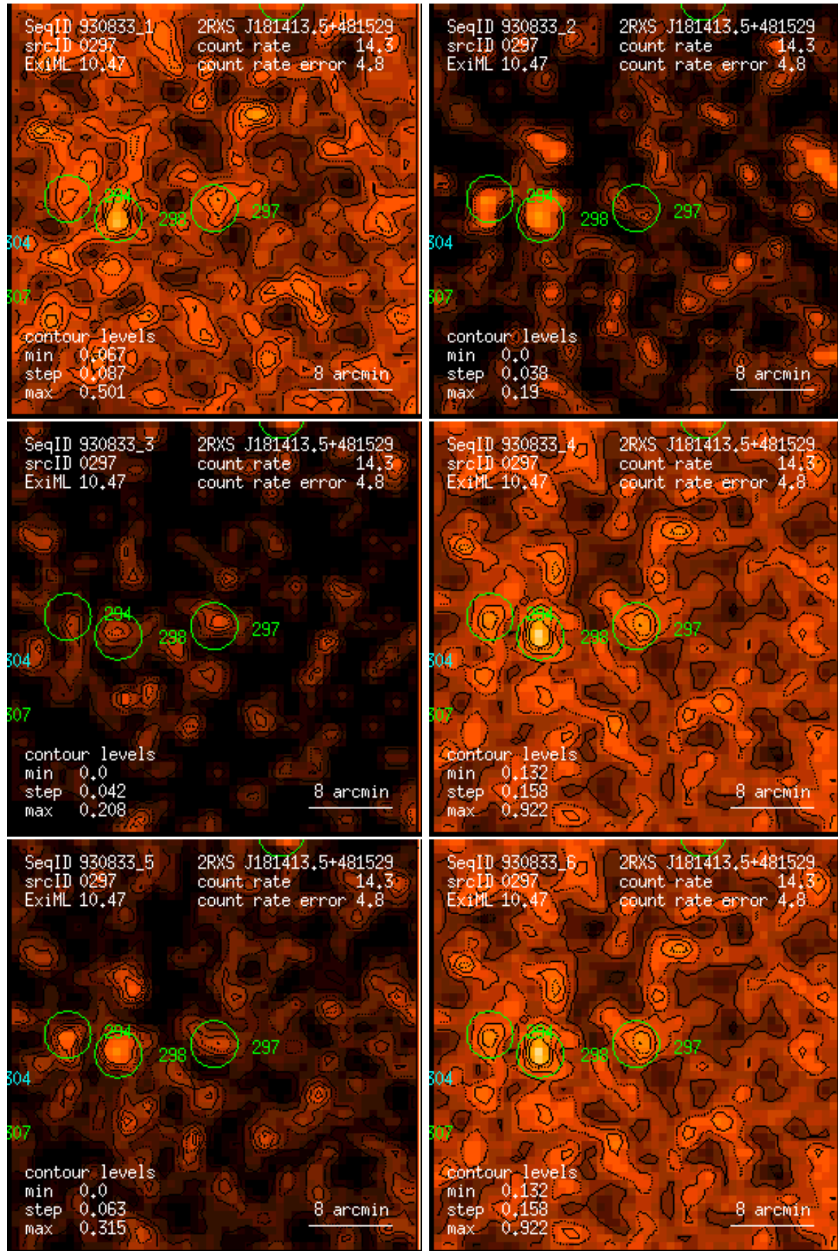
Figure 297: RASS 930833: detection 0297: band rate images, Gaussian filter: (1) PSPC channels 11 – 41, (2) 52 – 90, (3) 91 – 201, (4) 11 – 235, (5) 52 – 201, (6) 11 – 201. Broad band rates in counts/ks. Band rate contour levels in counts/ks/arcmin 2 .
