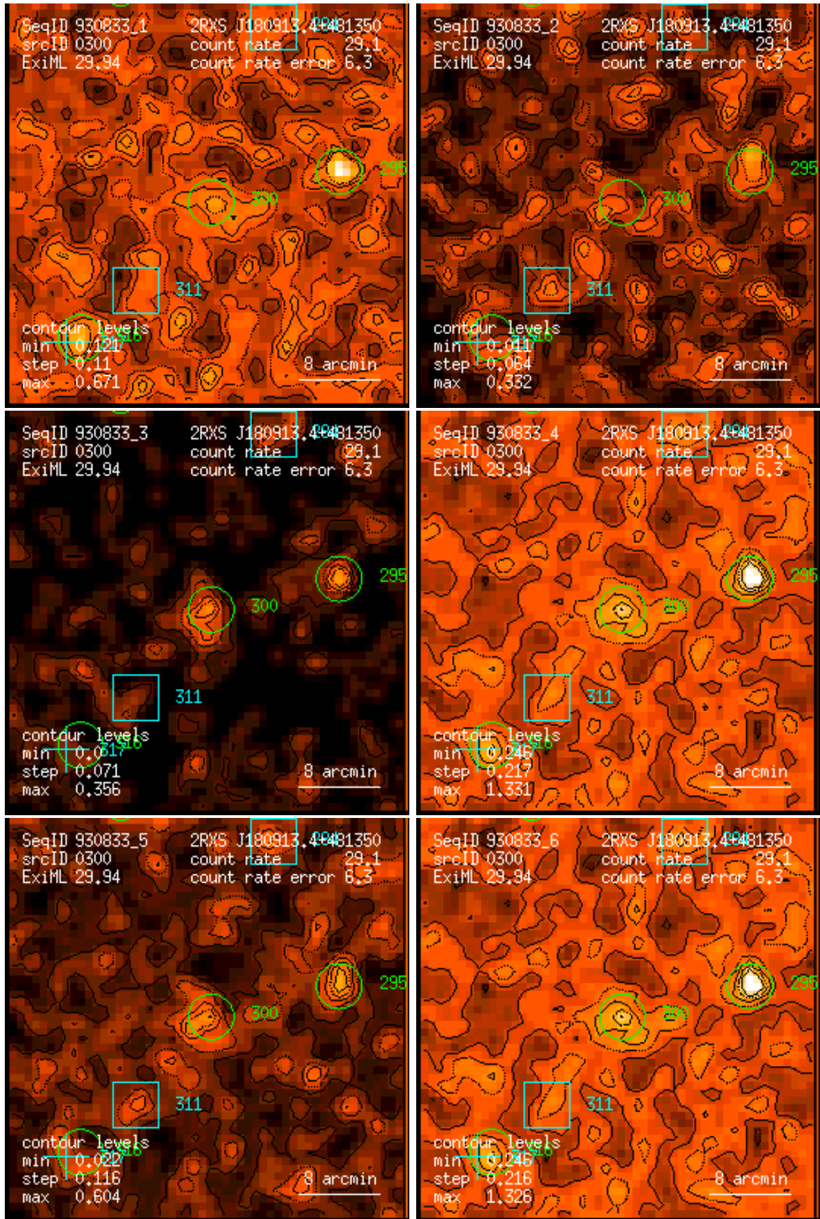
Figure 300: RASS 930833: detection 0300: band rate images, Gaussian filter: (1) PSPC channels 11 – 41, (2) 52 – 90, (3) 91 – 201, (4) 11 – 235, (5) 52 – 201, (6) 11 – 201. Broad band rates in counts/ks. Band rate contour levels in counts/ks/arcmin 2 .
