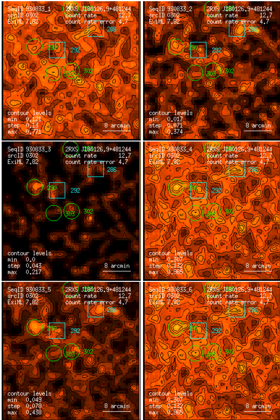
Figure 302: RASS 930833: detection 0302: band rate images, Gaussian filter: (1) PSPC channels 11 – 41, (2) 52 – 90, (3) 91 – 201, (4) 11 – 235, (5) 52 – 201, (6) 11 – 201. Broad band rates in counts/ks. Band rate contour levels in counts/ks/arcmin 2 .
