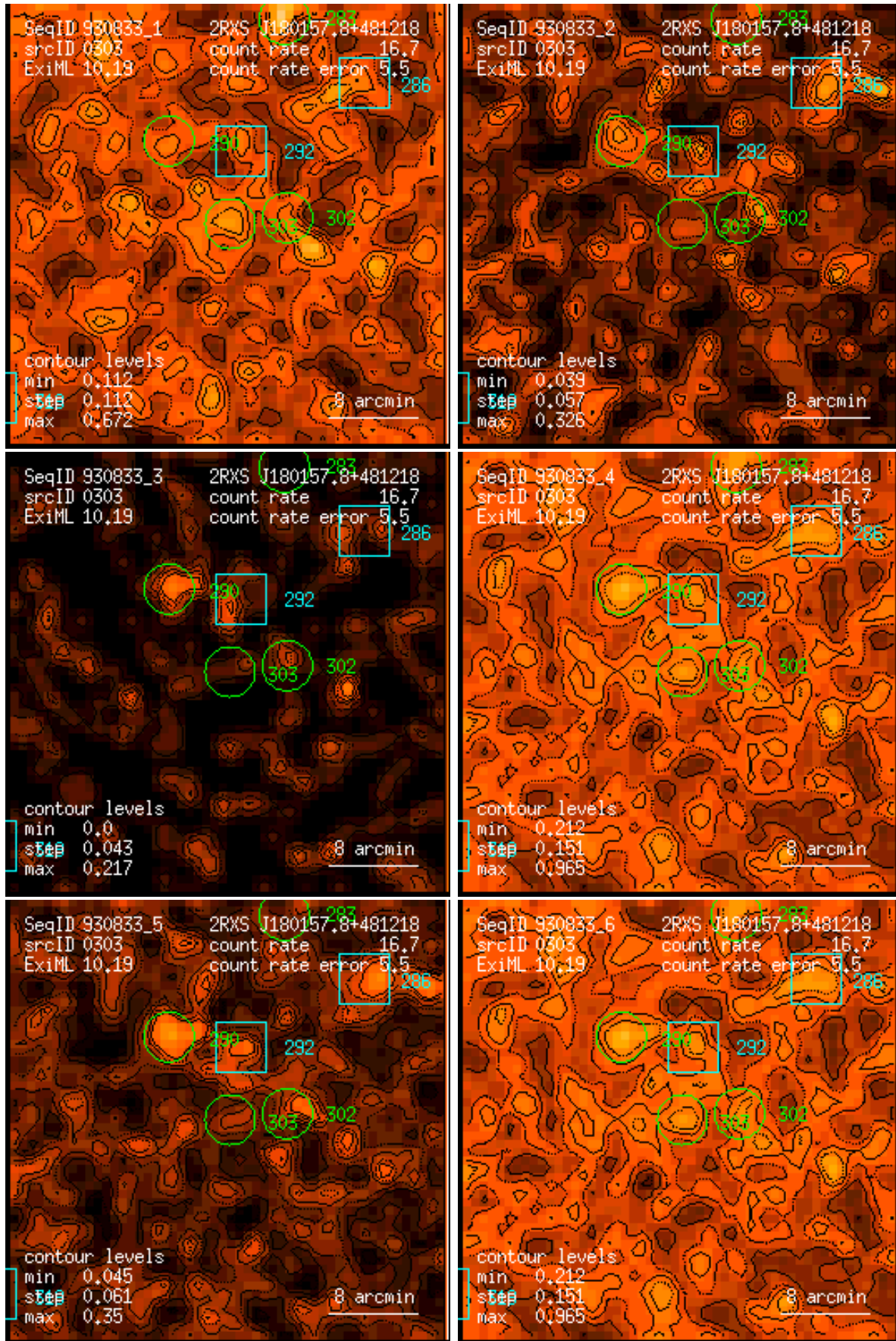
Figure 303: RASS 930833: detection 0303: band rate images, Gaussian filter: (1) PSPC channels 11 – 41, (2) 52 – 90, (3) 91 – 201, (4) 11 – 235, (5) 52 – 201, (6) 11 – 201. Broad band rates in counts/ks. Band rate contour levels in counts/ks/arcmin 2 .
