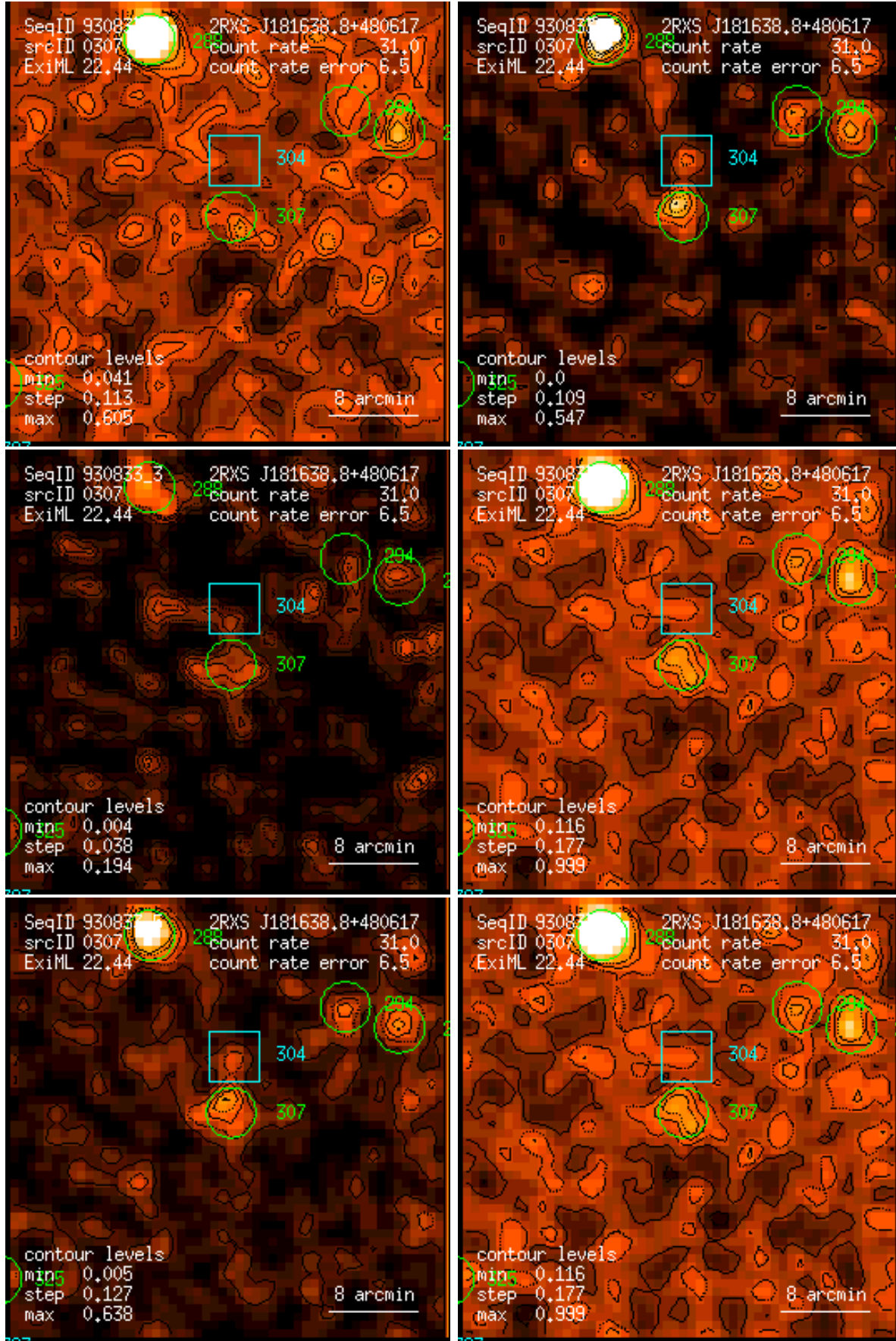
Figure 307: RASS 930833: detection 0307: band rate images, Gaussian filter: (1) PSPC channels 11 – 41, (2) 52 – 90, (3) 91 – 201, (4) 11 – 235, (5) 52 – 201, (6) 11 – 201. Broad band rates in counts/ks. Band rate contour levels in counts/ks/arcmin 2 .
