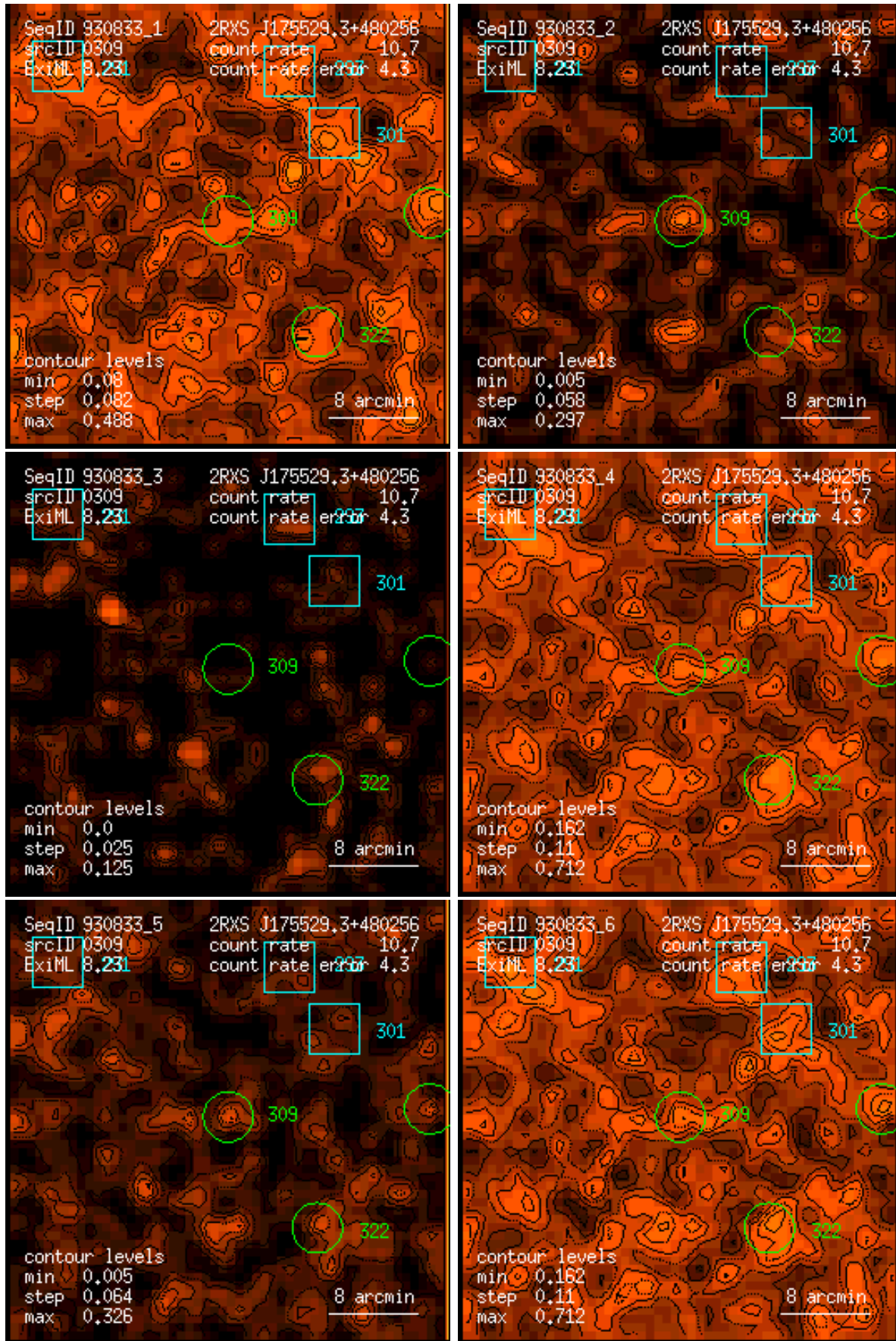
Figure 309: RASS 930833: detection 0309: band rate images, Gaussian filter: (1) PSPC channels 11 – 41, (2) 52 – 90, (3) 91 – 201, (4) 11 – 235, (5) 52 – 201, (6) 11 – 201. Broad band rates in counts/ks. Band rate contour levels in counts/ks/arcmin 2 .
