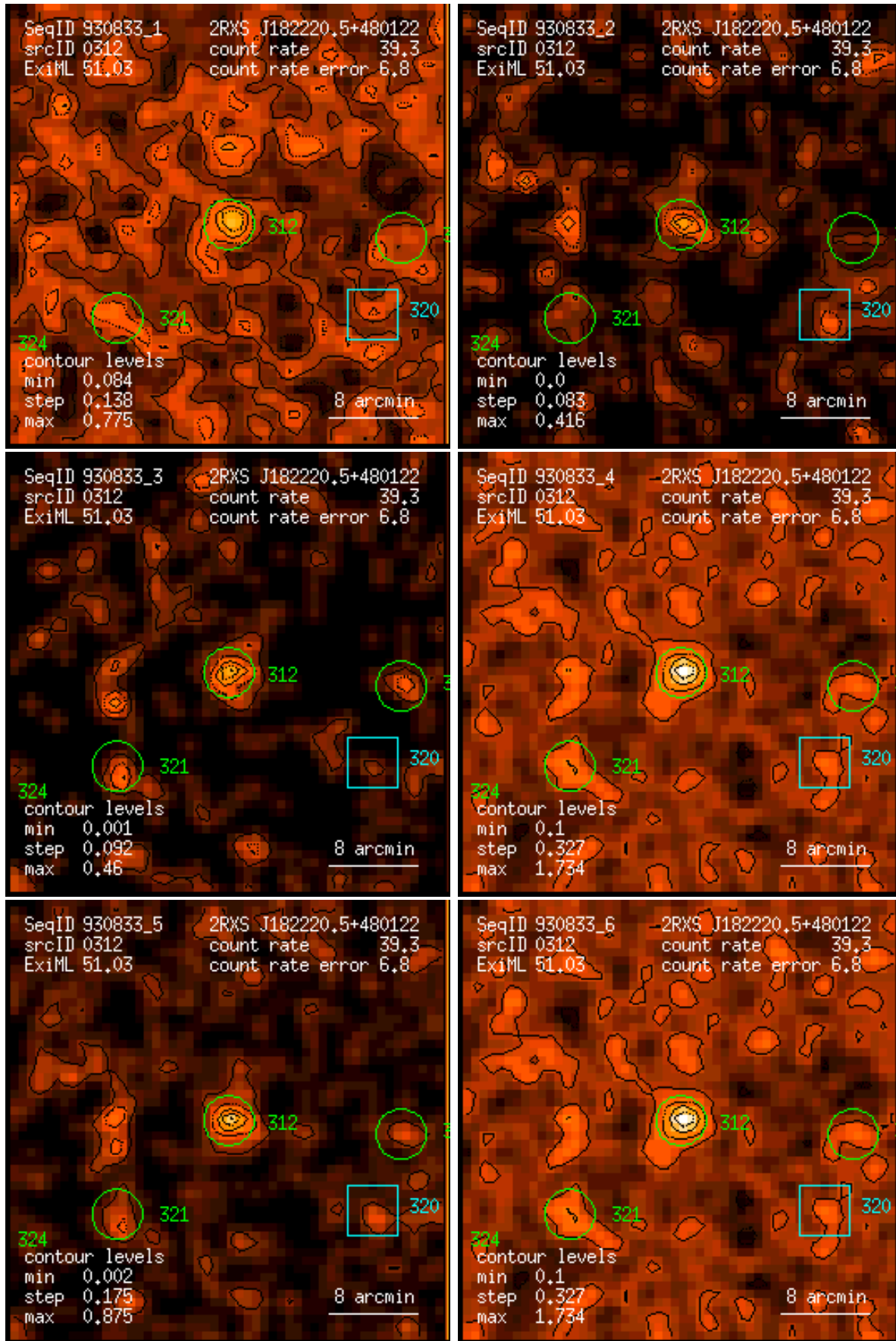
Figure 312: RASS 930833: detection 0312: band rate images, Gaussian filter: (1) PSPC channels 11 – 41, (2) 52 – 90, (3) 91 – 201, (4) 11 – 235, (5) 52 – 201, (6) 11 – 201. Broad band rates in counts/ks. Band rate contour levels in counts/ks/arcmin 2 .
