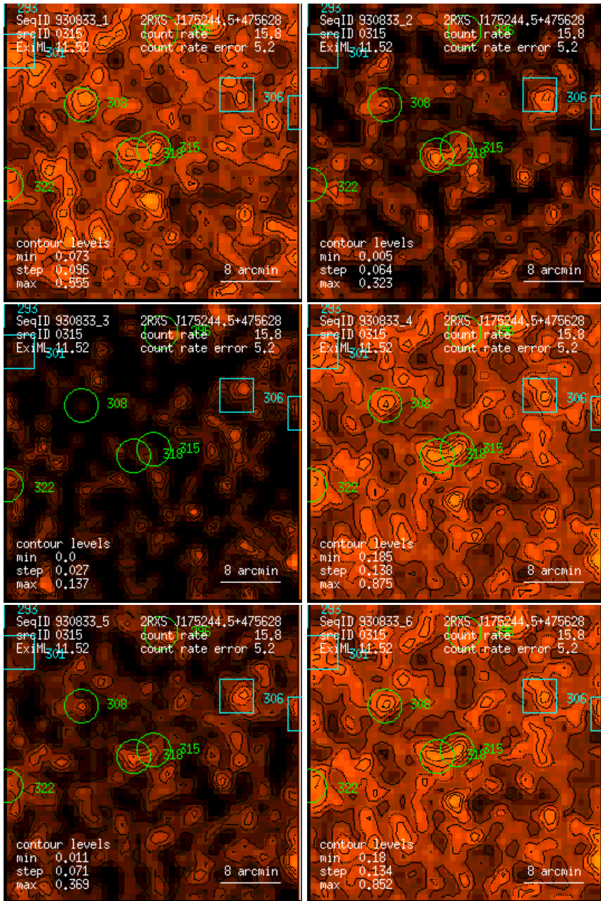
Figure 315: RASS 930833: detection 0315: band rate images, Gaussian filter: (1) PSPC channels 11 – 41, (2) 52 – 90, (3) 91 – 201, (4) 11 – 235, (5) 52 – 201, (6) 11 – 201. Broad band rates in counts/ks. Band rate contour levels in counts/ks/arcmin 2 .
