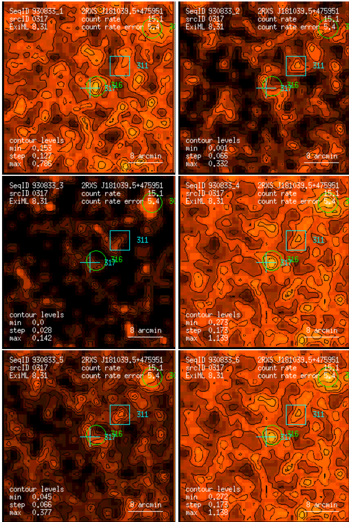
Figure 317: RASS 930833: detection 0317: band rate images, Gaussian filter: (1) PSPC channels 11 – 41, (2) 52 – 90, (3) 91 – 201, (4) 11 – 235, (5) 52 – 201, (6) 11 – 201. Broad band rates in counts/ks. Band rate contour levels in counts/ks/arcmin 2 .
