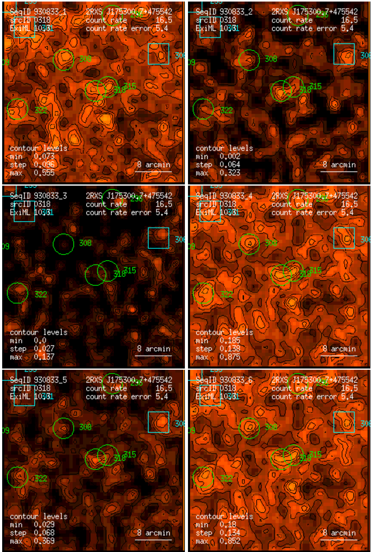
Figure 318: RASS 930833: detection 0318: band rate images, Gaussian filter: (1) PSPC channels 11 – 41, (2) 52 – 90, (3) 91 – 201, (4) 11 – 235, (5) 52 – 201, (6) 11 – 201. Broad band rates in counts/ks. Band rate contour levels in counts/ks/arcmin 2 .
