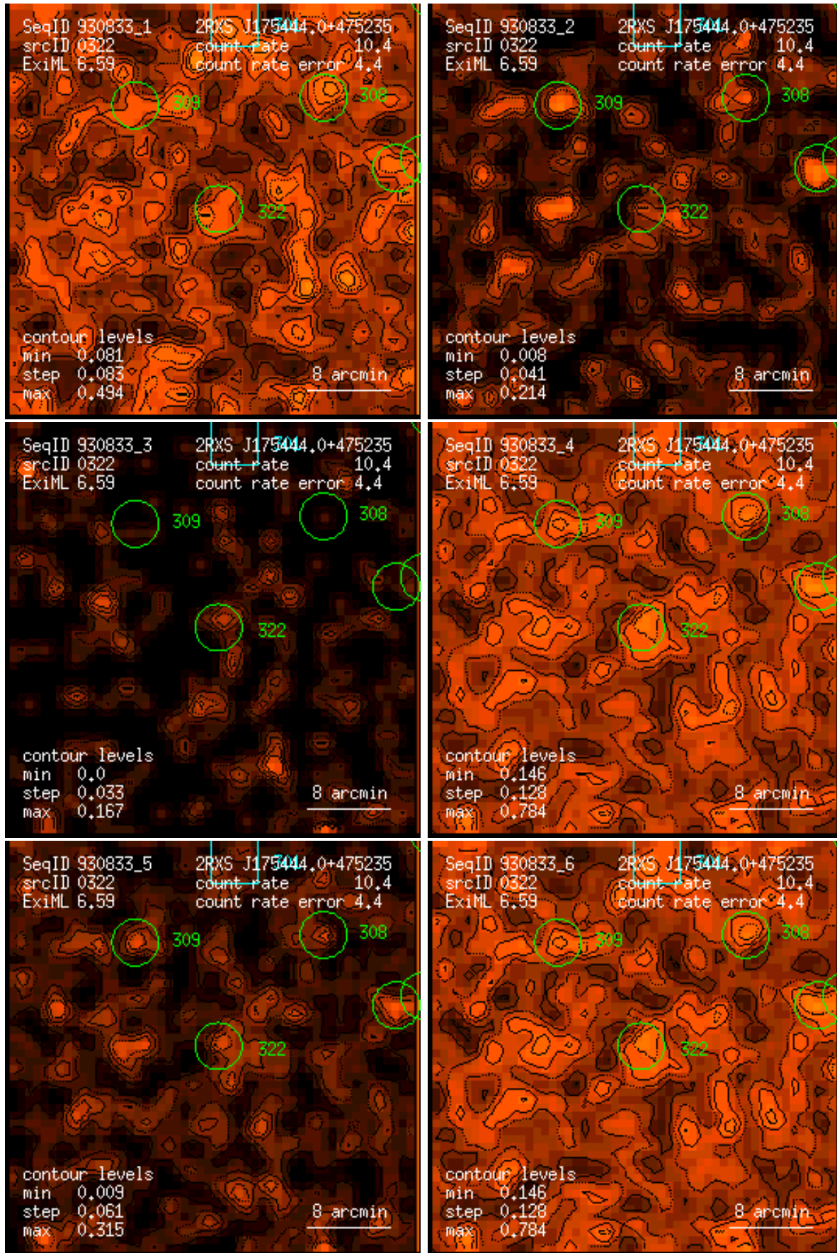
Figure 322: RASS 930833: detection 0322: band rate images, Gaussian filter: (1) PSPC channels 11 – 41, (2) 52 – 90, (3) 91 – 201, (4) 11 – 235, (5) 52 – 201, (6) 11 – 201. Broad band rates in counts/ks. Band rate contour levels in counts/ks/arcmin 2 .
