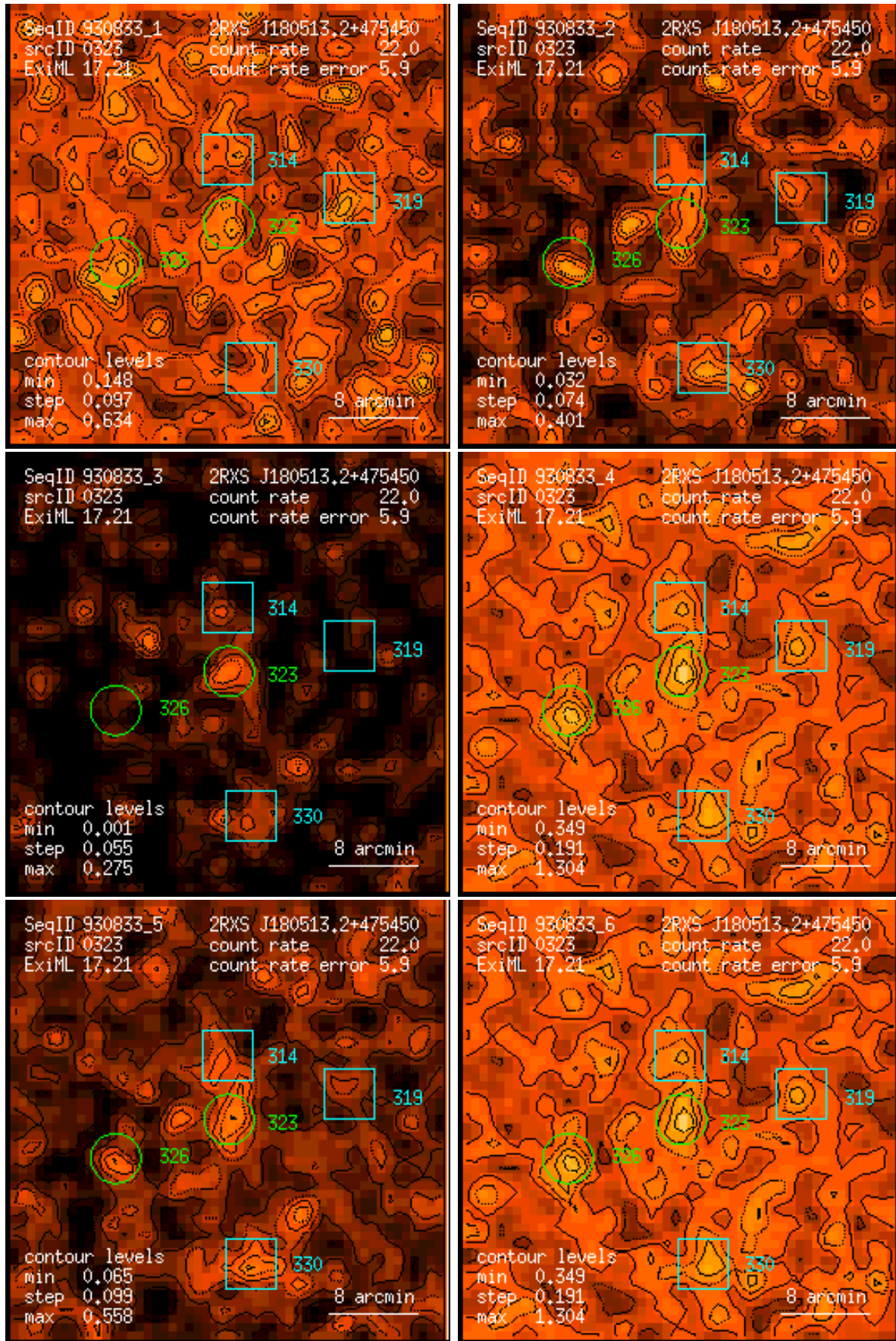
Figure 323: RASS 930833: detection 0323: band rate images, Gaussian filter: (1) PSPC channels 11 – 41, (2) 52 – 90, (3) 91 – 201, (4) 11 – 235, (5) 52 – 201, (6) 11 – 201. Broad band rates in counts/ks. Band rate contour levels in counts/ks/arcmin 2 .
