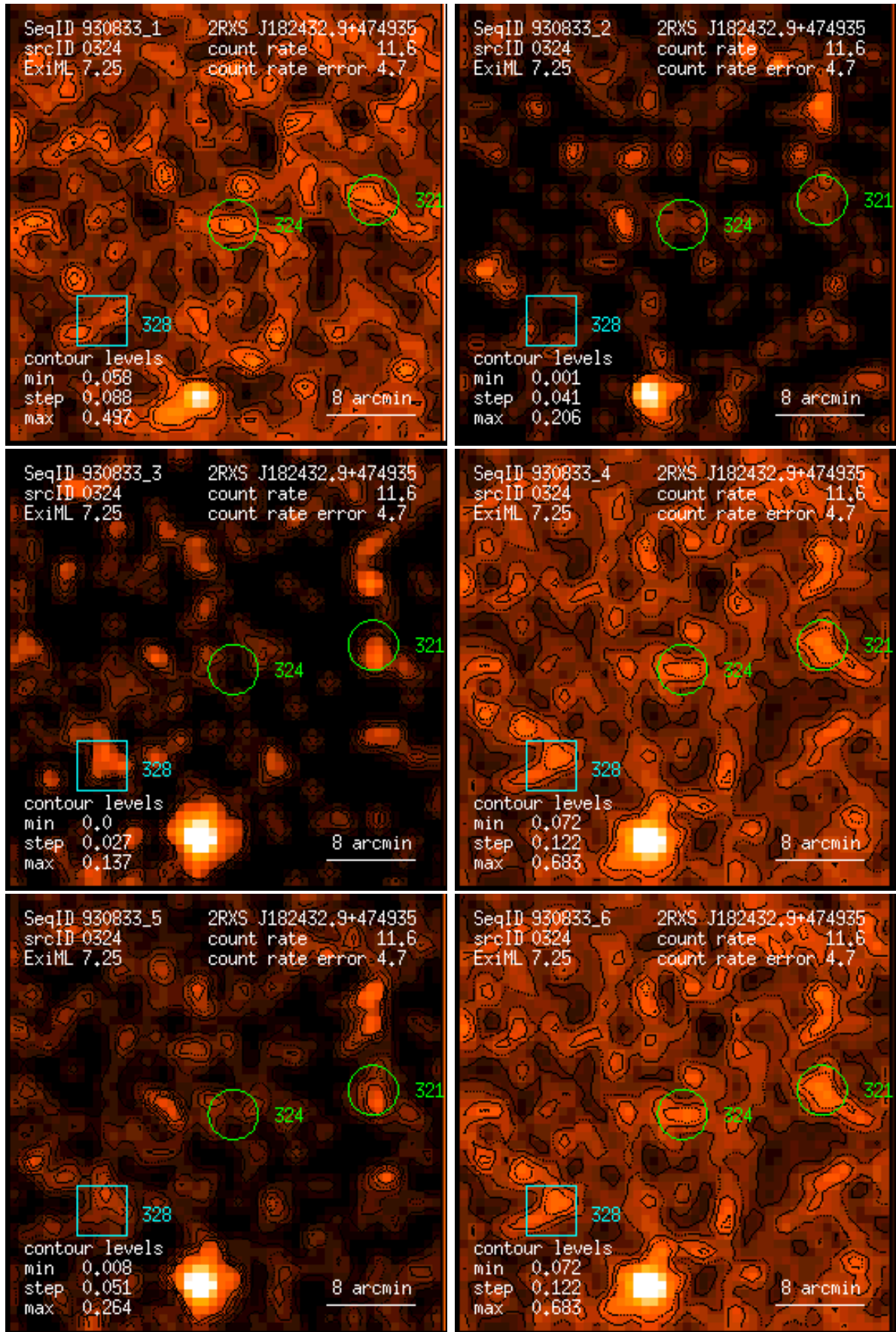
Figure 324: RASS 930833: detection 0324: band rate images, Gaussian filter: (1) PSPC channels 11 – 41, (2) 52 – 90, (3) 91 – 201, (4) 11 – 235, (5) 52 – 201, (6) 11 – 201. Broad band rates in counts/ks. Band rate contour levels in counts/ks/arcmin 2 .
