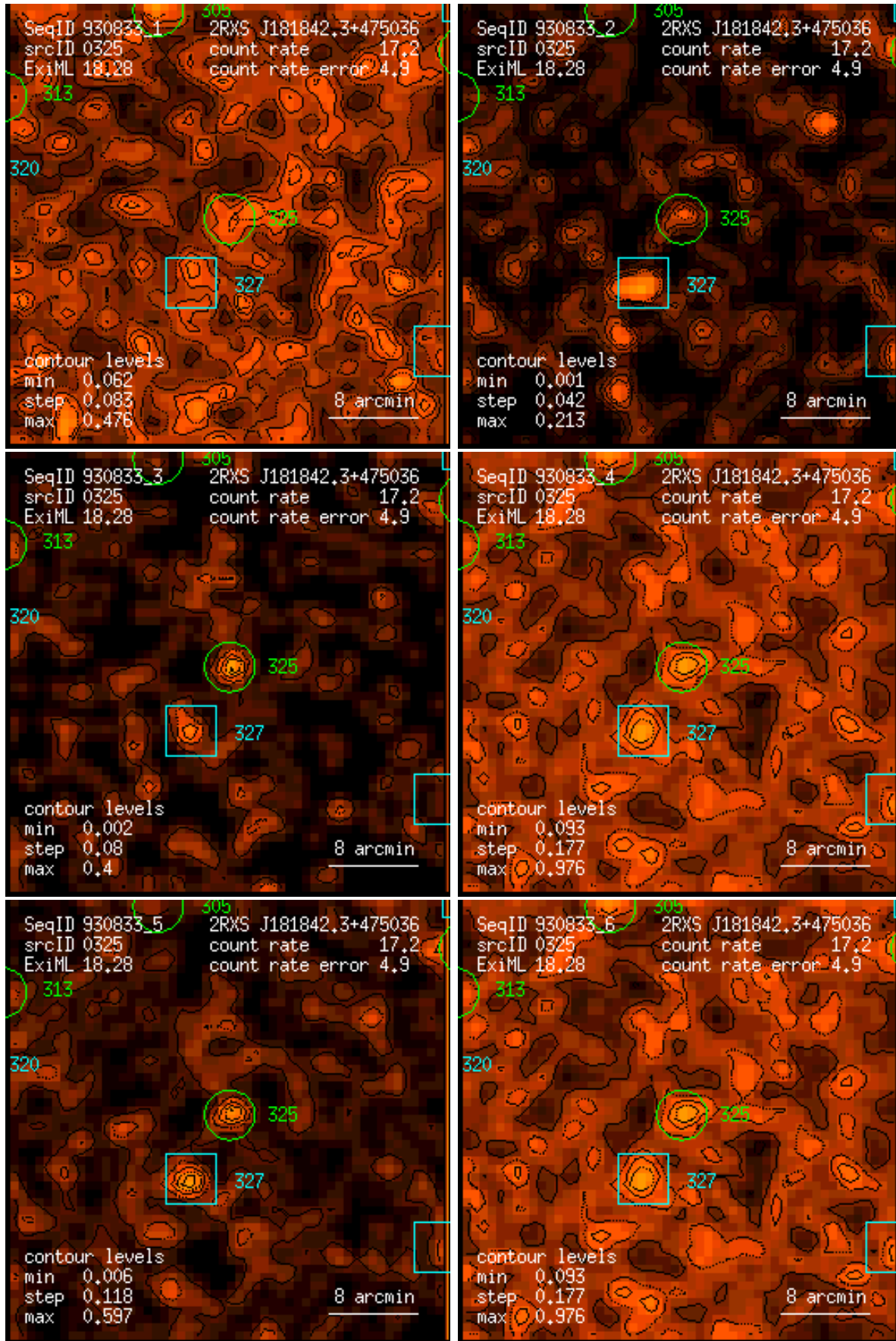
Figure 325: RASS 930833: detection 0325: band rate images, Gaussian filter: (1) PSPC channels 11 – 41, (2) 52 – 90, (3) 91 – 201, (4) 11 – 235, (5) 52 – 201, (6) 11 – 201. Broad band rates in counts/ks. Band rate contour levels in counts/ks/arcmin 2 .
