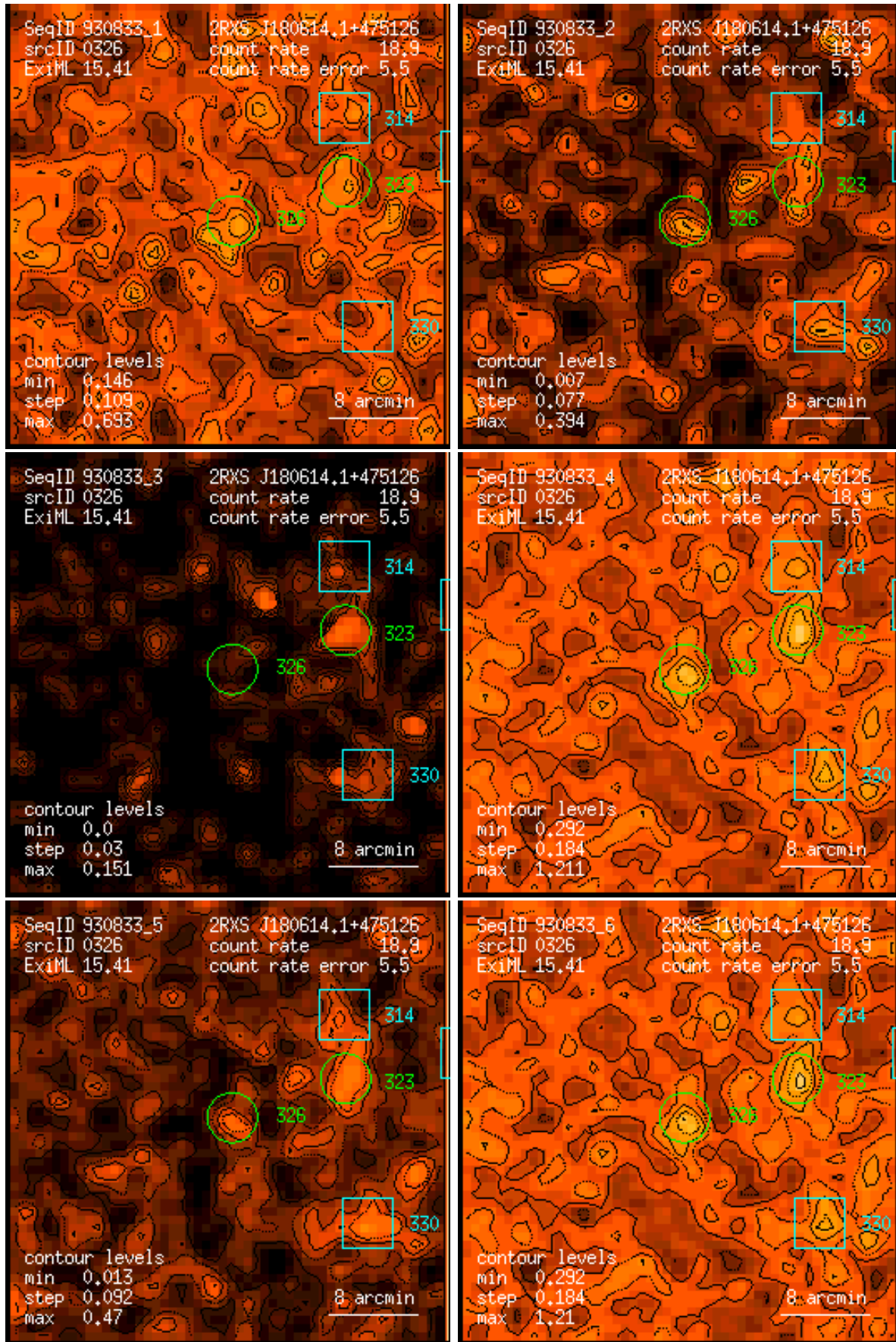
Figure 326: RASS 930833: detection 0326: band rate images, Gaussian filter: (1) PSPC channels 11 – 41, (2) 52 – 90, (3) 91 – 201, (4) 11 – 235, (5) 52 – 201, (6) 11 – 201. Broad band rates in counts/ks. Band rate contour levels in counts/ks/arcmin 2 .
