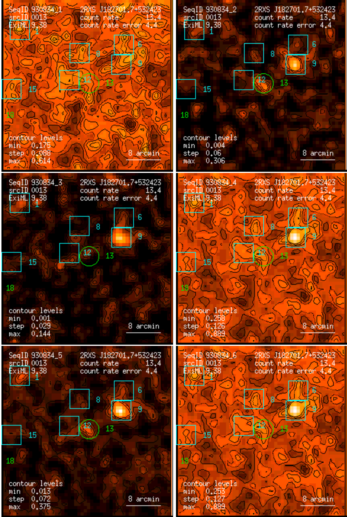
Figure 13: RASS 930834: detection 0013: band rate images, Gaussian filter: (1) PSPC channels 11 – 41, (2) 52 – 90, (3) 91 – 201, (4) 11 – 235, (5) 52 – 201, (6) 11 – 201. Broad band rates in counts/ks. Band rate contour levels in counts/ks/arcmin 2 .
