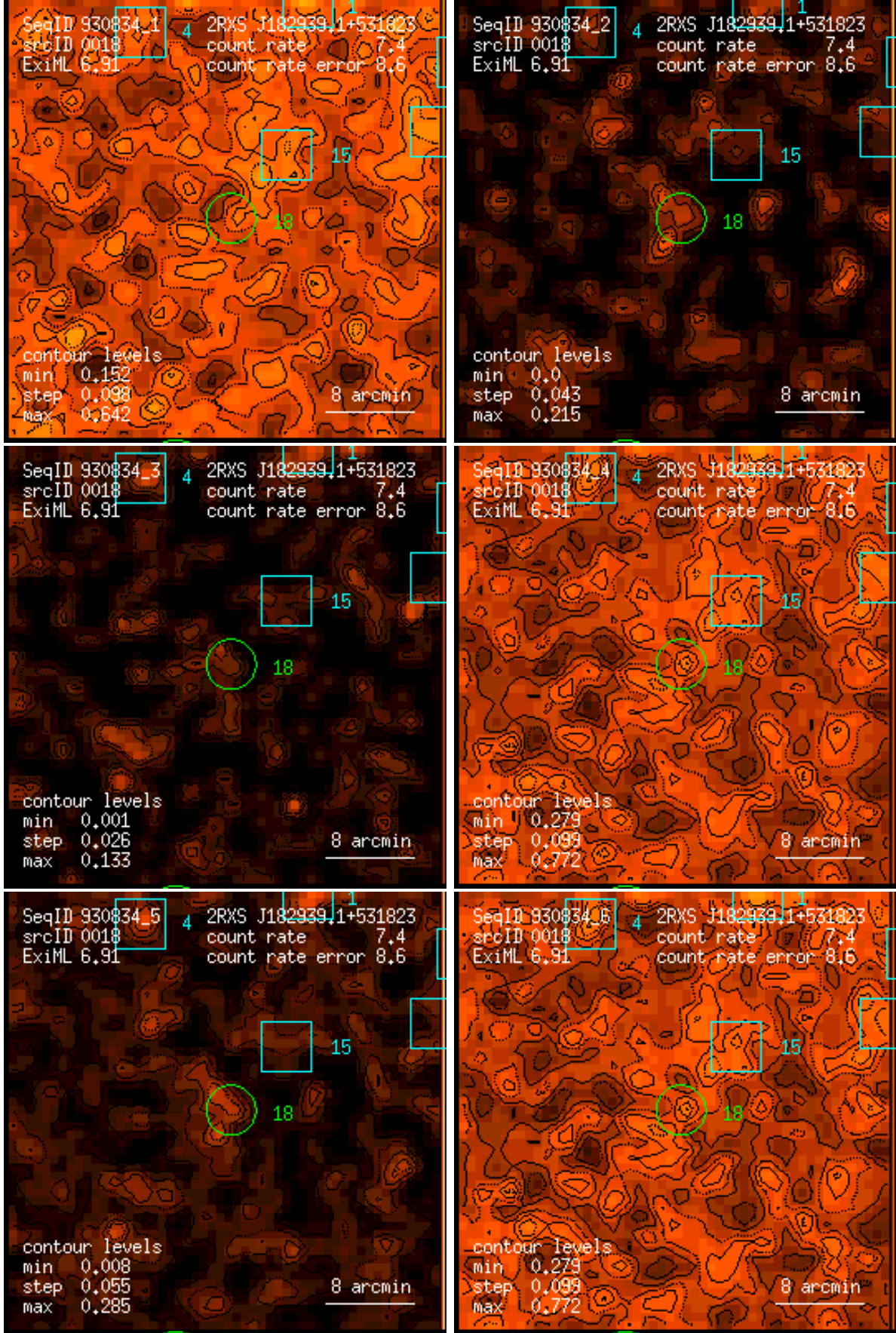
Figure 18: RASS 930834: detection 0018: band rate images, Gaussian filter: (1) PSPC channels 11 – 41, (2) 52 – 90, (3) 91 – 201, (4) 11 – 235, (5) 52 – 201, (6) 11 – 201. Broad band rates in counts/ks. Band rate contour levels in counts/ks/arcmin 2 .
