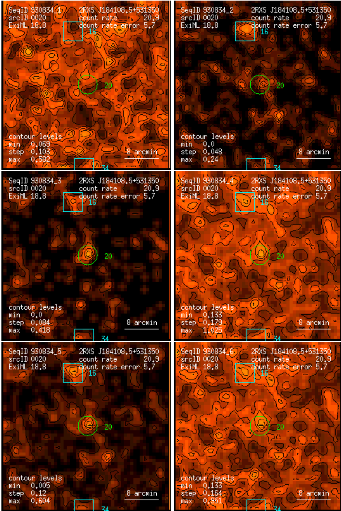
Figure 20: RASS 930834: detection 0020: band rate images, Gaussian filter: (1) PSPC channels 11 – 41, (2) 52 – 90, (3) 91 – 201, (4) 11 – 235, (5) 52 – 201, (6) 11 – 201. Broad band rates in counts/ks. Band rate contour levels in counts/ks/arcmin 2 .
