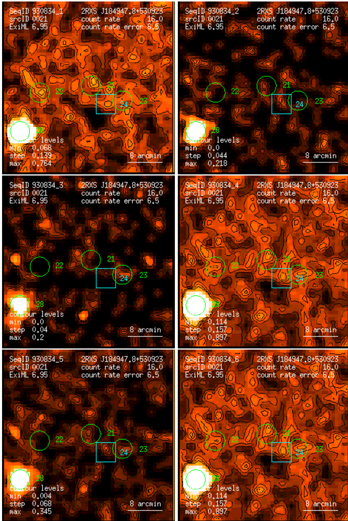
Figure 21: RASS 930834: detection 0021: band rate images, Gaussian filter: (1) PSPC channels 11 – 41, (2) 52 – 90, (3) 91 – 201, (4) 11 – 235, (5) 52 – 201, (6) 11 – 201. Broad band rates in counts/ks. Band rate contour levels in counts/ks/arcmin 2 .
