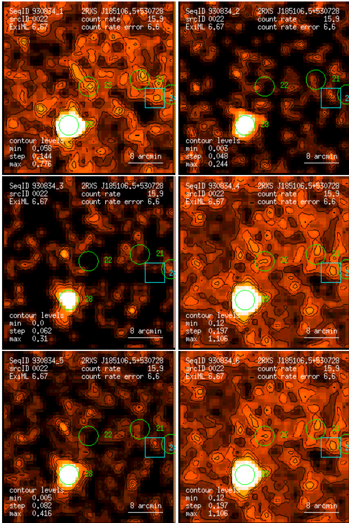
Figure 22: RASS 930834: detection 0022: band rate images, Gaussian filter: (1) PSPC channels 11 – 41, (2) 52 – 90, (3) 91 – 201, (4) 11 – 235, (5) 52 – 201, (6) 11 – 201. Broad band rates in counts/ks. Band rate contour levels in counts/ks/arcmin 2 .
