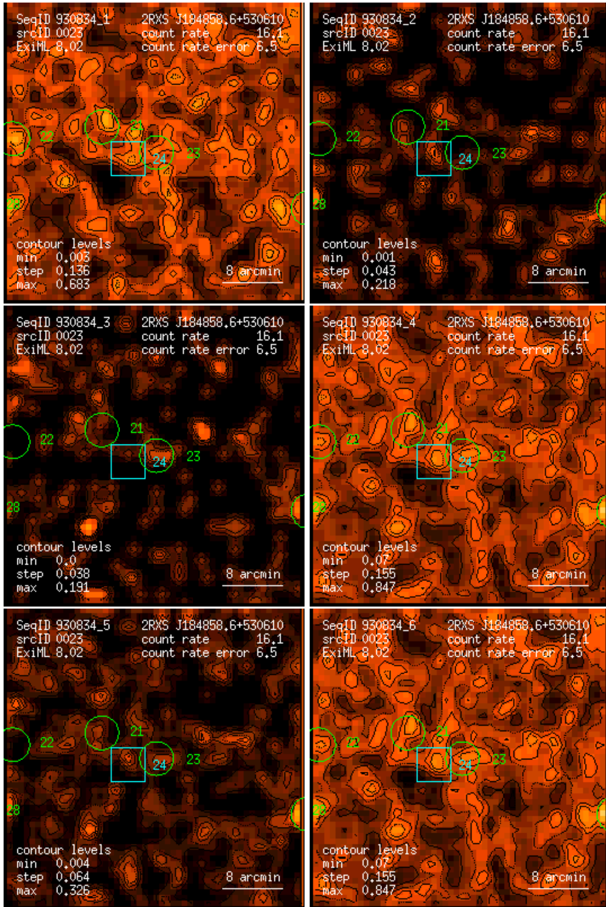
Figure 23: RASS 930834: detection 0023: band rate images, Gaussian filter: (1) PSPC channels 11 – 41, (2) 52 – 90, (3) 91 – 201, (4) 11 – 235, (5) 52 – 201, (6) 11 – 201. Broad band rates in counts/ks. Band rate contour levels in counts/ks/arcmin 2 .
