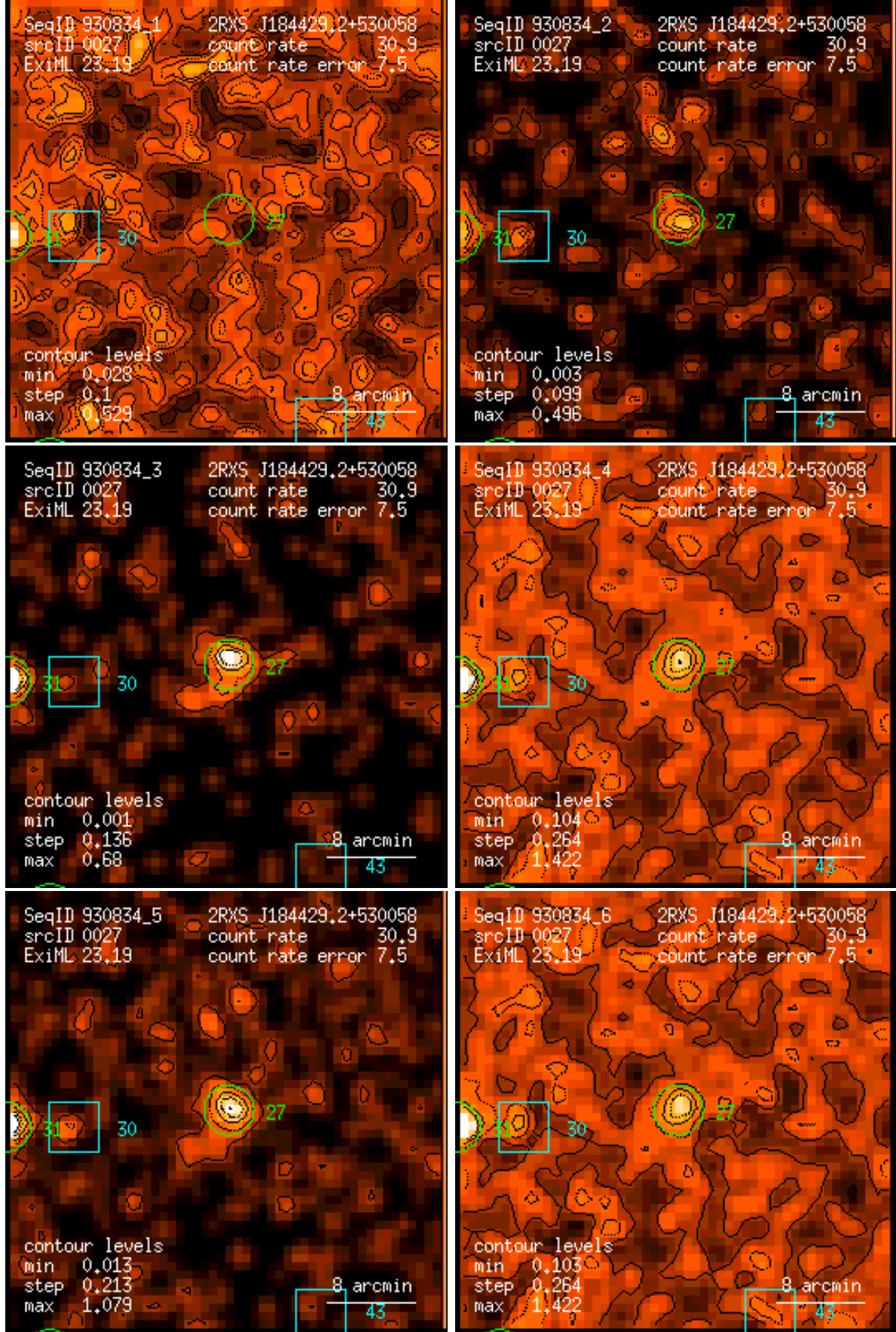
Figure 27: RASS 930834: detection 0027: band rate images, Gaussian filter: (1) PSPC channels 11 – 41, (2) 52 – 90, (3) 91 – 201, (4) 11 – 235, (5) 52 – 201, (6) 11 – 201. Broad band rates in counts/ks. Band rate contour levels in counts/ks/arcmin 2 .
