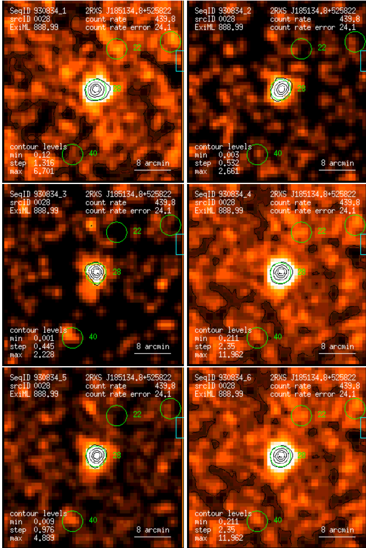
Figure 28: RASS 930834: detection 0028: band rate images, Gaussian filter: (1) PSPC channels 11 – 41, (2) 52 – 90, (3) 91 – 201, (4) 11 – 235, (5) 52 – 201, (6) 11 – 201. Broad band rates in counts/ks. Band rate contour levels in counts/ks/arcmin 2 .
