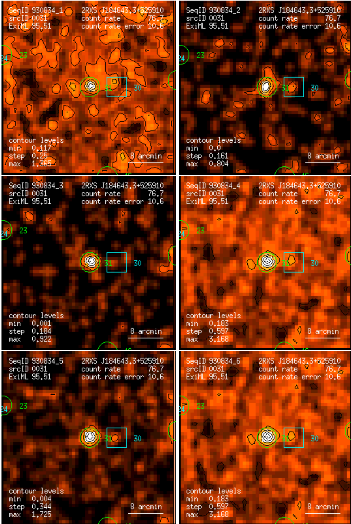
Figure 31: RASS 930834: detection 0031: band rate images, Gaussian filter: (1) PSPC channels 11 – 41, (2) 52 – 90, (3) 91 – 201, (4) 11 – 235, (5) 52 – 201, (6) 11 – 201. Broad band rates in counts/ks. Band rate contour levels in counts/ks/arcmin 2 .
