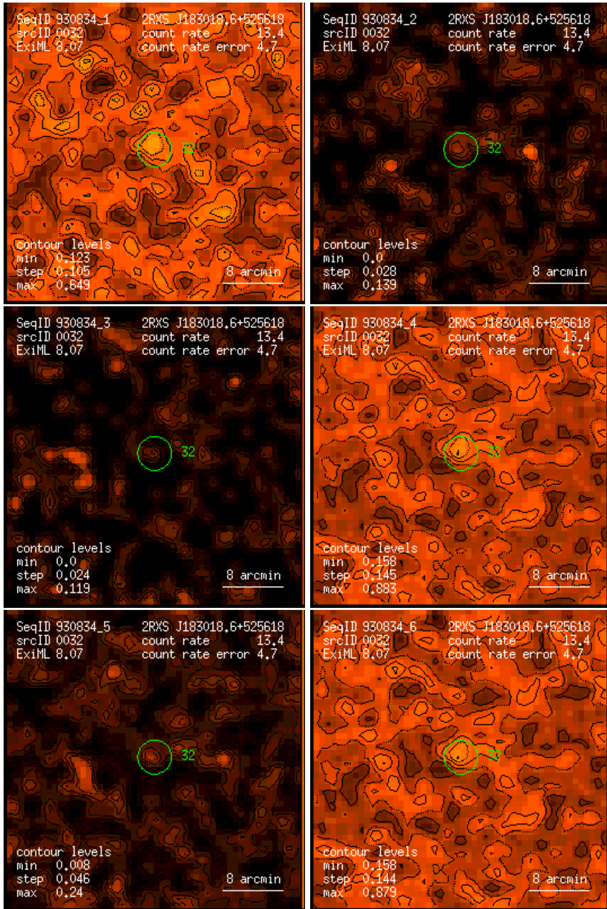
Figure 32: RASS 930834: detection 0032: band rate images, Gaussian filter: (1) PSPC channels 11 – 41, (2) 52 – 90, (3) 91 – 201, (4) 11 – 235, (5) 52 – 201, (6) 11 – 201. Broad band rates in counts/ks. Band rate contour levels in counts/ks/arcmin 2 .
