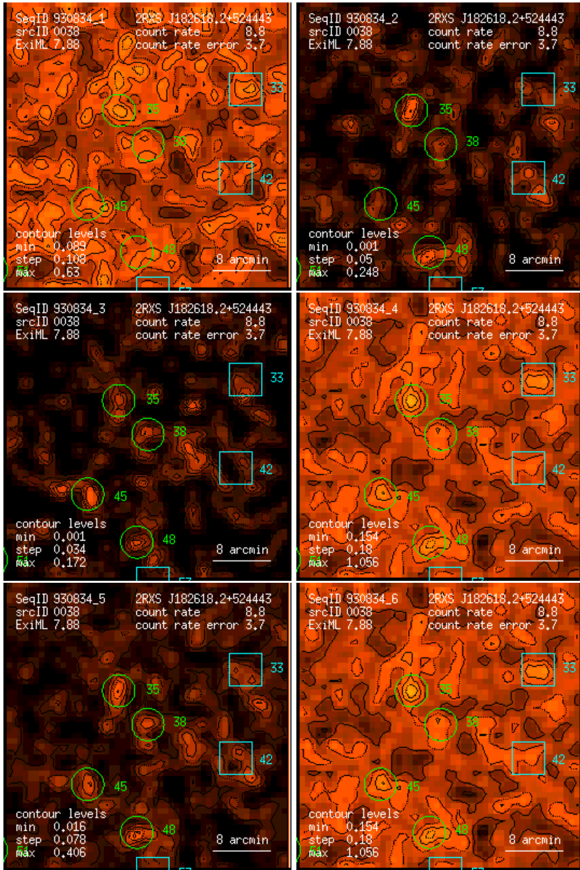
Figure 38: RASS 930834: detection 0038: band rate images, Gaussian filter: (1) PSPC channels 11 – 41, (2) 52 – 90, (3) 91 – 201, (4) 11 – 235, (5) 52 – 201, (6) 11 – 201. Broad band rates in counts/ks. Band rate contour levels in counts/ks/arcmin 2 .
