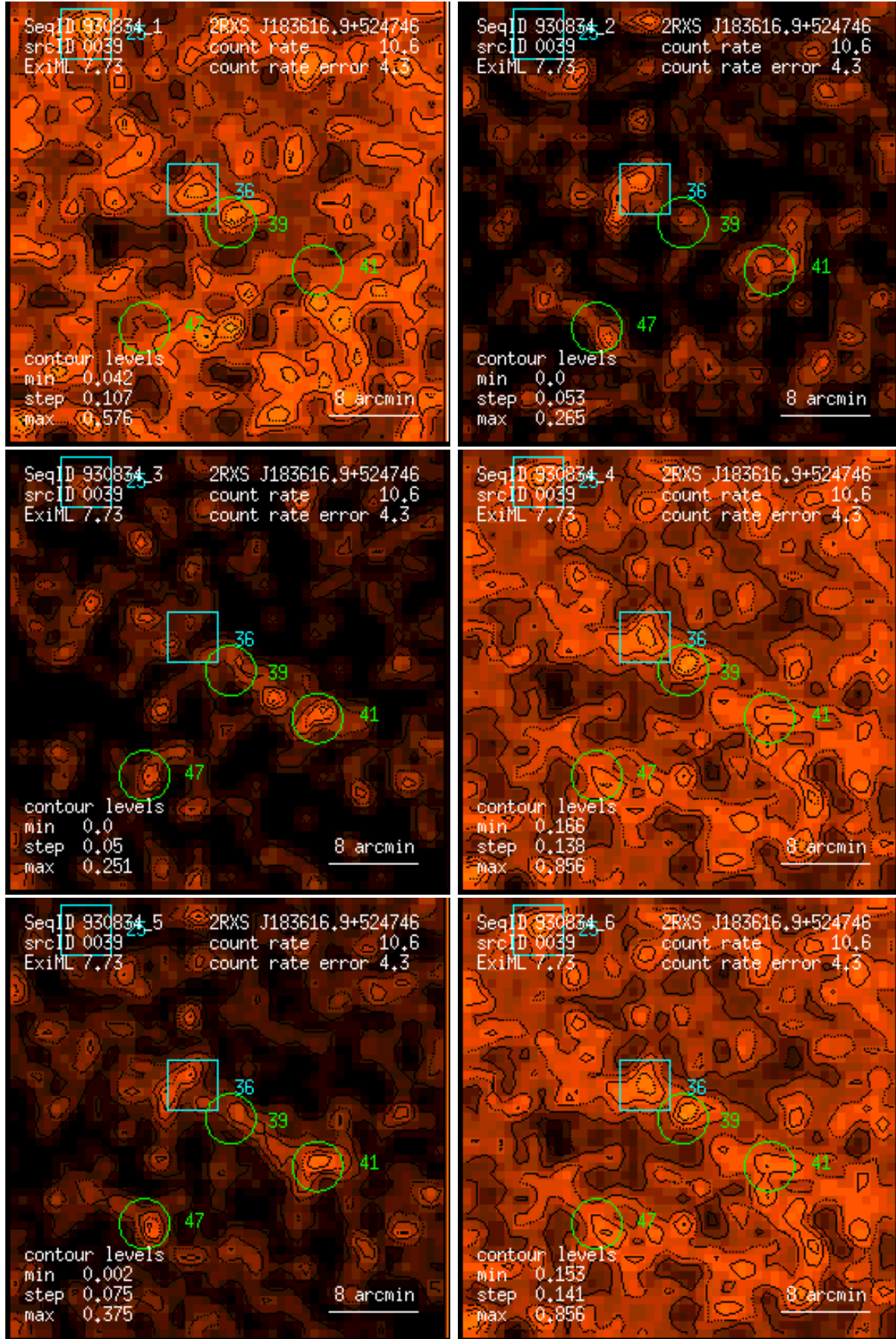
Figure 39: RASS 930834: detection 0039: band rate images, Gaussian filter: (1) PSPC channels 11 – 41, (2) 52 – 90, (3) 91 – 201, (4) 11 – 235, (5) 52 – 201, (6) 11 – 201. Broad band rates in counts/ks. Band rate contour levels in counts/ks/arcmin 2 .
