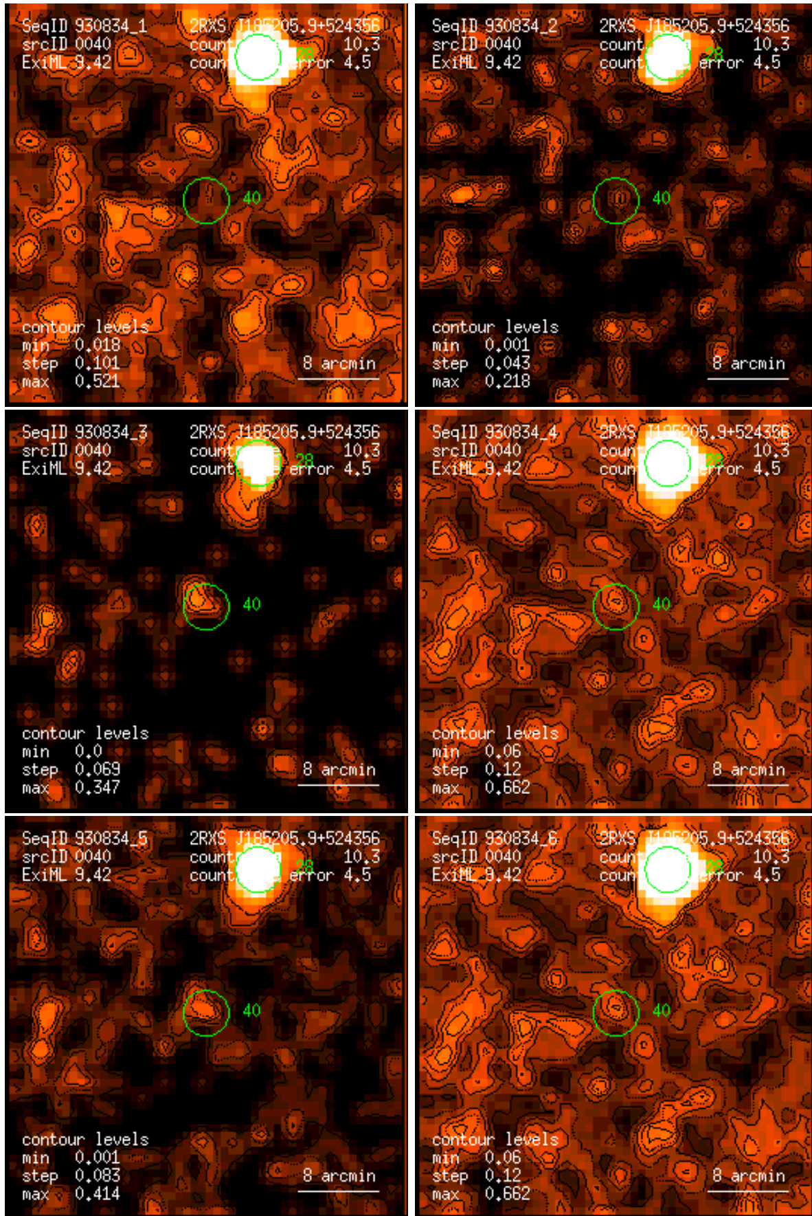
Figure 40: RASS 930834: detection 0040: band rate images, Gaussian filter: (1) PSPC channels 11 – 41, (2) 52 – 90, (3) 91 – 201, (4) 11 – 235, (5) 52 – 201, (6) 11 – 201. Broad band rates in counts/ks. Band rate contour levels in counts/ks/arcmin 2 .
