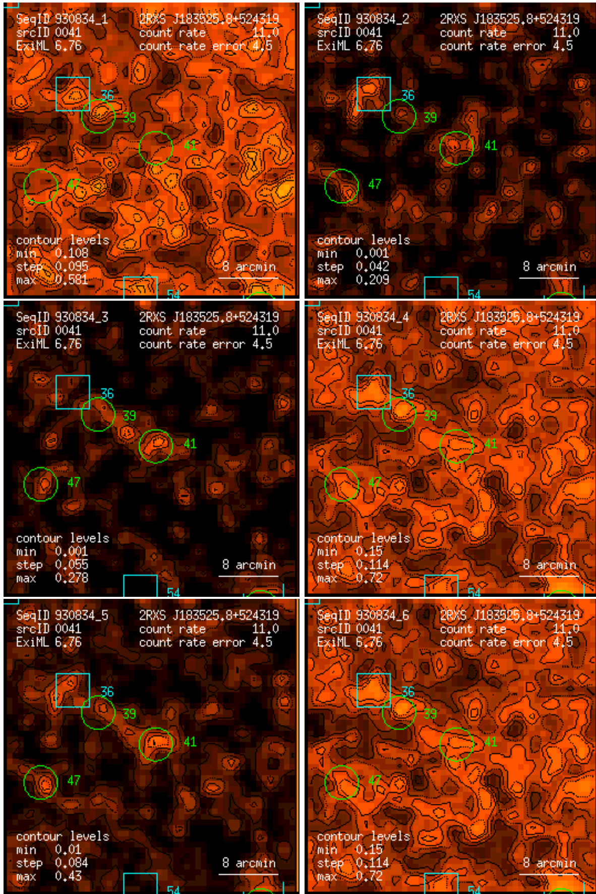
Figure 41: RASS 930834: detection 0041: band rate images, Gaussian filter: (1) PSPC channels 11 – 41, (2) 52 – 90, (3) 91 – 201, (4) 11 – 235, (5) 52 – 201, (6) 11 – 201. Broad band rates in counts/ks. Band rate contour levels in counts/ks/arcmin 2 .
