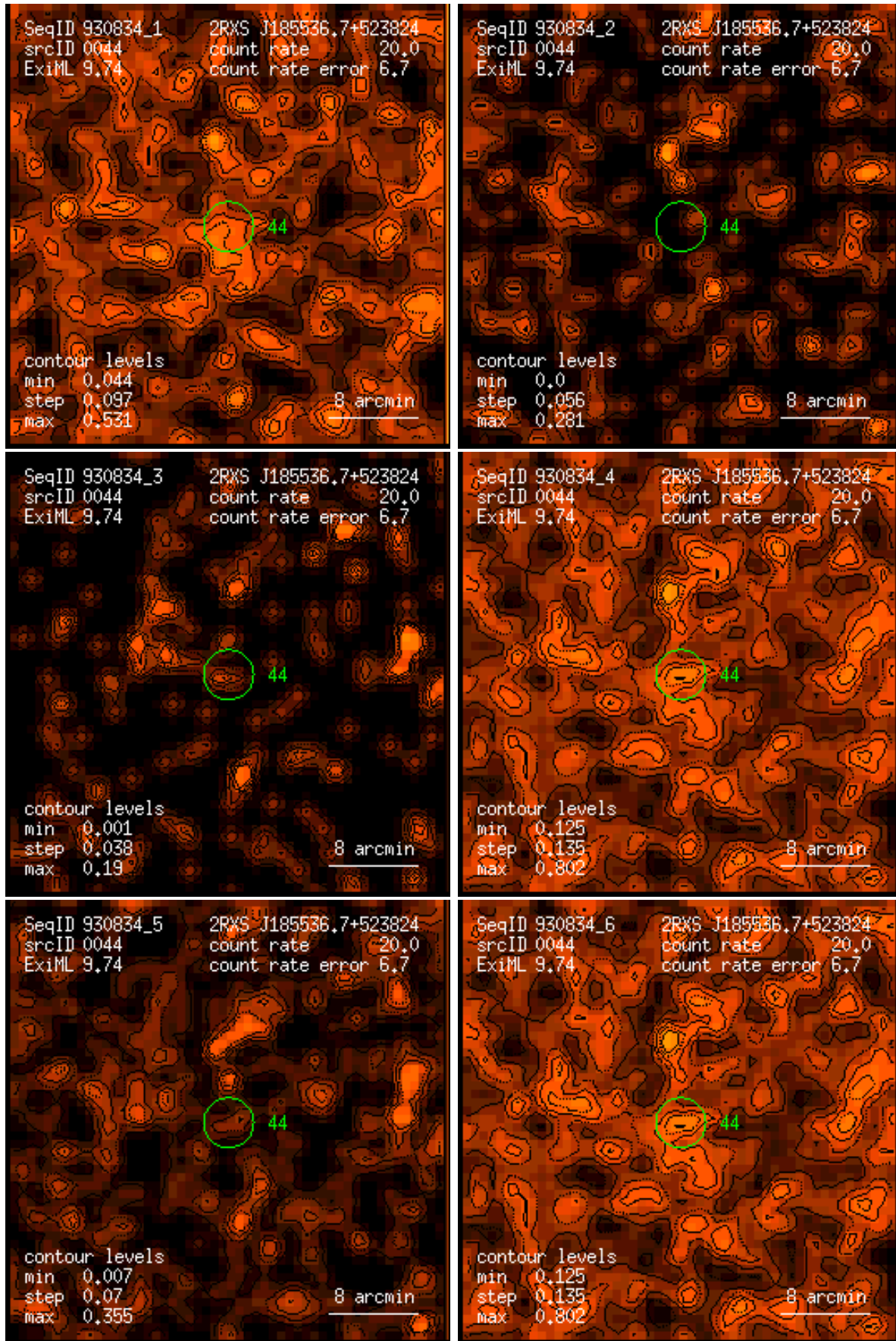
Figure 44: RASS 930834: detection 0044: band rate images, Gaussian filter: (1) PSPC channels 11 – 41, (2) 52 – 90, (3) 91 – 201, (4) 11 – 235, (5) 52 – 201, (6) 11 – 201. Broad band rates in counts/ks. Band rate contour levels in counts/ks/arcmin 2 .
