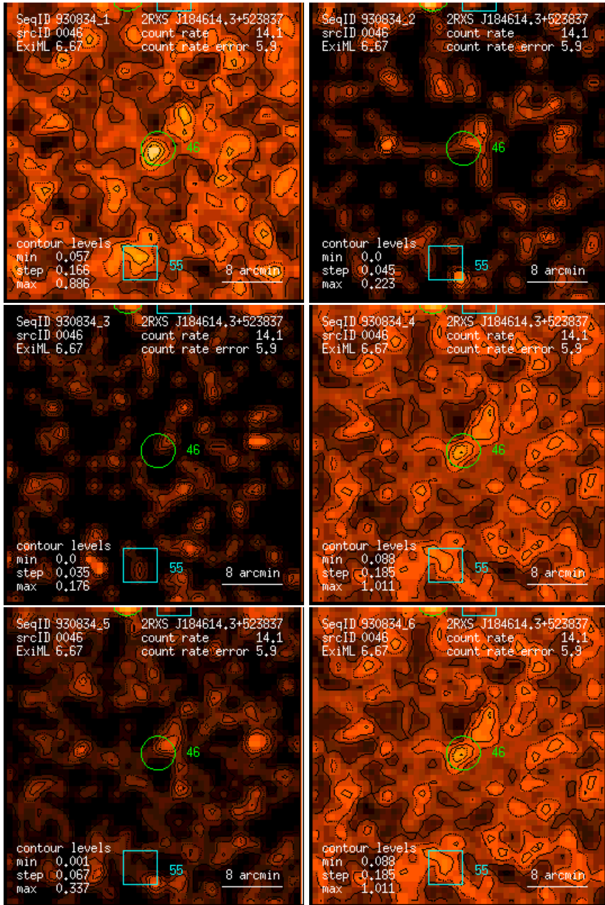
Figure 46: RASS 930834: detection 0046: band rate images, Gaussian filter: (1) PSPC channels 11 – 41, (2) 52 – 90, (3) 91 – 201, (4) 11 – 235, (5) 52 – 201, (6) 11 – 201. Broad band rates in counts/ks. Band rate contour levels in counts/ks/arcmin 2 .
