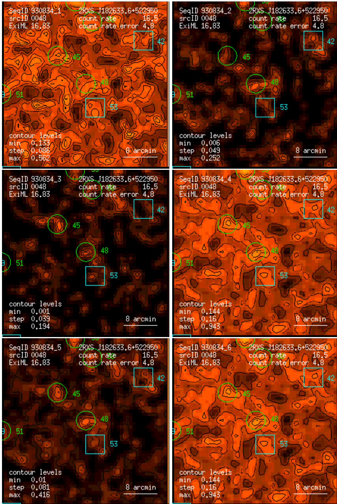
Figure 48: RASS 930834: detection 0048: band rate images, Gaussian filter: (1) PSPC channels 11 – 41, (2) 52 – 90, (3) 91 – 201, (4) 11 – 235, (5) 52 – 201, (6) 11 – 201. Broad band rates in counts/ks. Band rate contour levels in counts/ks/arcmin 2 .
