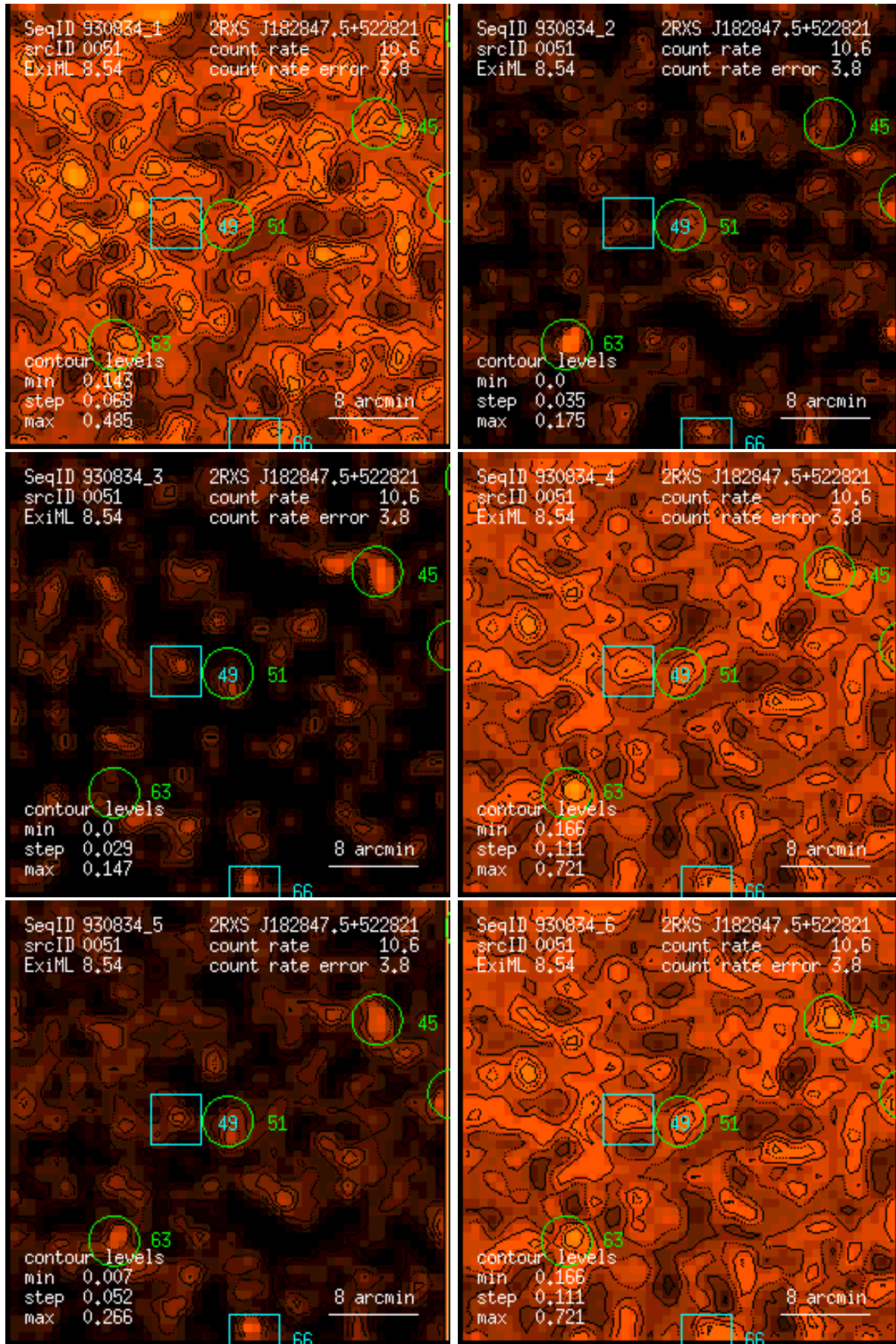
Figure 51: RASS 930834: detection 0051: band rate images, Gaussian filter: (1) PSPC channels 11 – 41, (2) 52 – 90, (3) 91 – 201, (4) 11 – 235, (5) 52 – 201, (6) 11 – 201. Broad band rates in counts/ks. Band rate contour levels in counts/ks/arcmin 2 .
