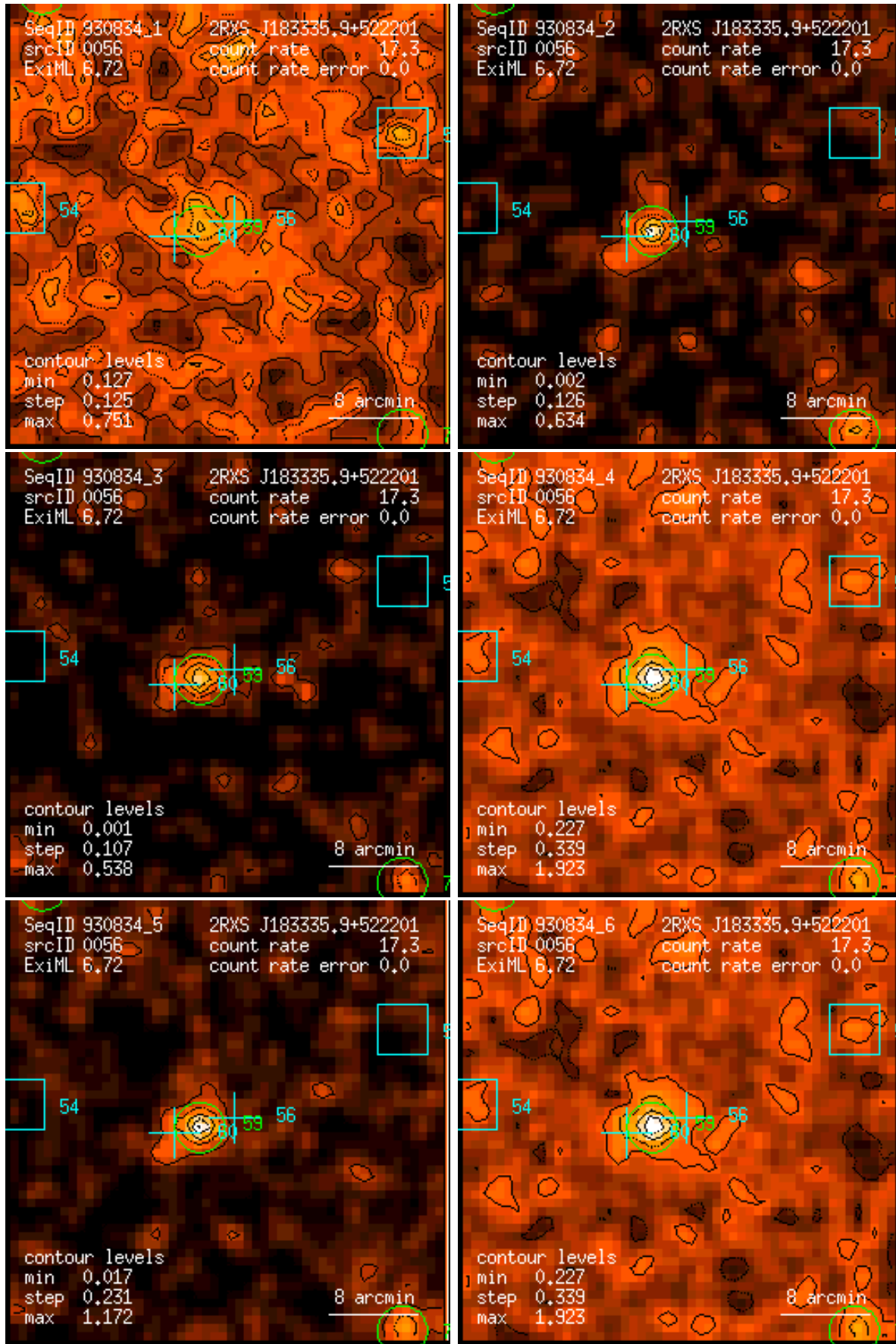
Figure 56: RASS 930834: detection 0056: band rate images, Gaussian filter: (1) PSPC channels 11 – 41, (2) 52 – 90, (3) 91 – 201, (4) 11 – 235, (5) 52 – 201, (6) 11 – 201. Broad band rates in counts/ks. Band rate contour levels in counts/ks/arcmin 2 .
