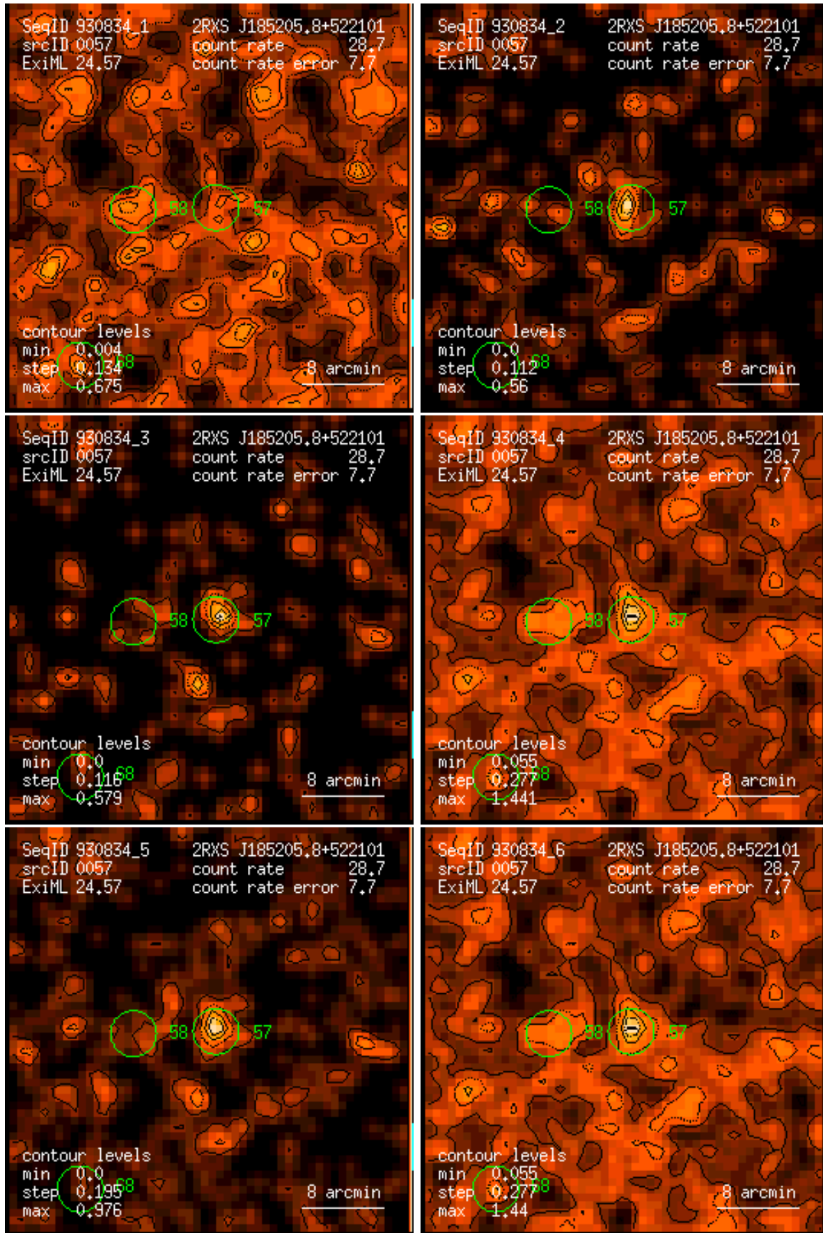
Figure 57: RASS 930834: detection 0057: band rate images, Gaussian filter: (1) PSPC channels 11 – 41, (2) 52 – 90, (3) 91 – 201, (4) 11 – 235, (5) 52 – 201, (6) 11 – 201. Broad band rates in counts/ks. Band rate contour levels in counts/ks/arcmin 2 .
