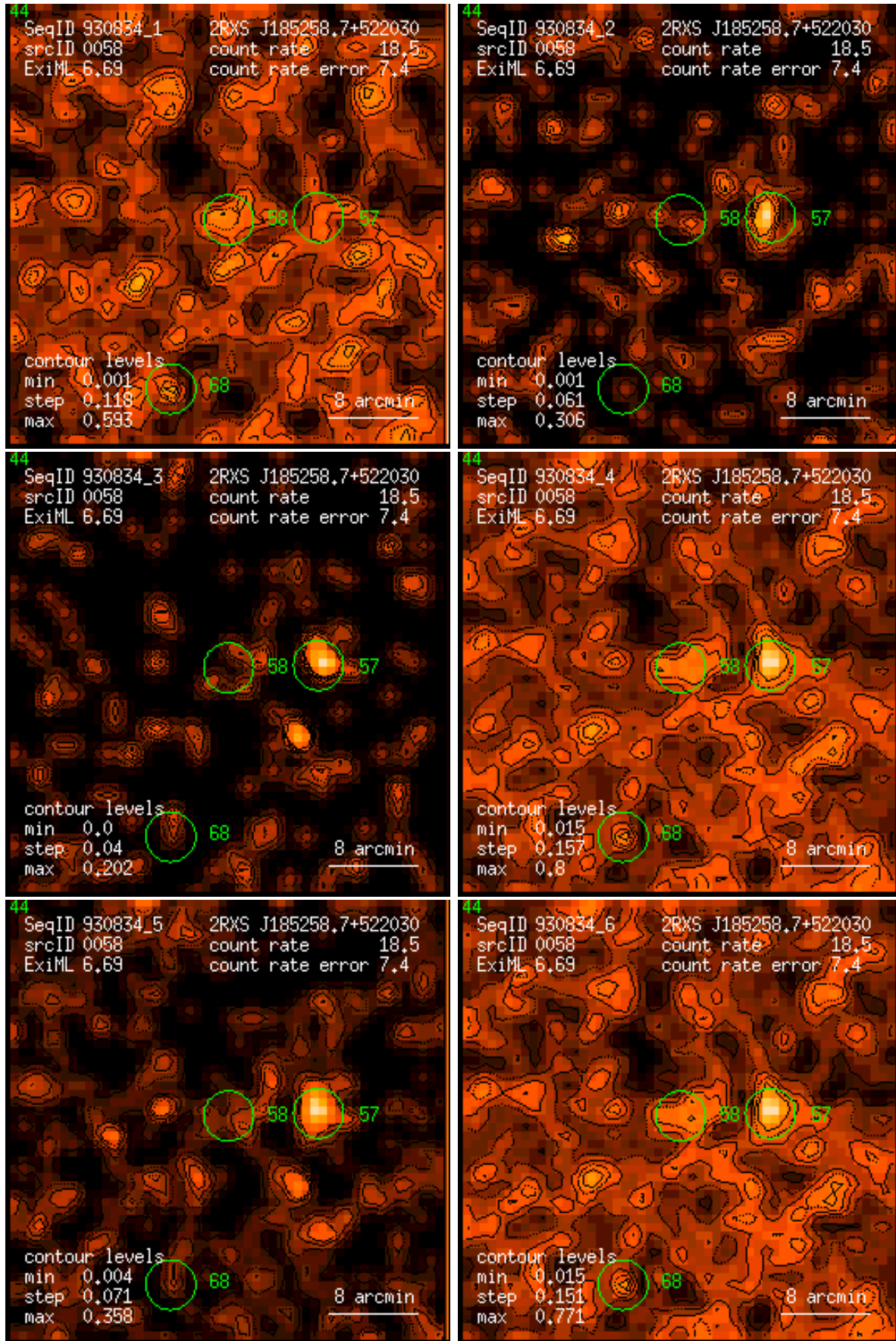
Figure 58: RASS 930834: detection 0058: band rate images, Gaussian filter: (1) PSPC channels 11 – 41, (2) 52 – 90, (3) 91 – 201, (4) 11 – 235, (5) 52 – 201, (6) 11 – 201. Broad band rates in counts/ks. Band rate contour levels in counts/ks/arcmin 2 .
