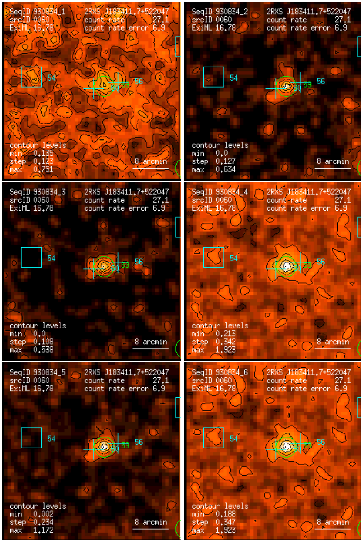
Figure 60: RASS 930834: detection 0060: band rate images, Gaussian filter: (1) PSPC channels 11 – 41, (2) 52 – 90, (3) 91 – 201, (4) 11 – 235, (5) 52 – 201, (6) 11 – 201. Broad band rates in counts/ks. Band rate contour levels in counts/ks/arcmin 2 .
