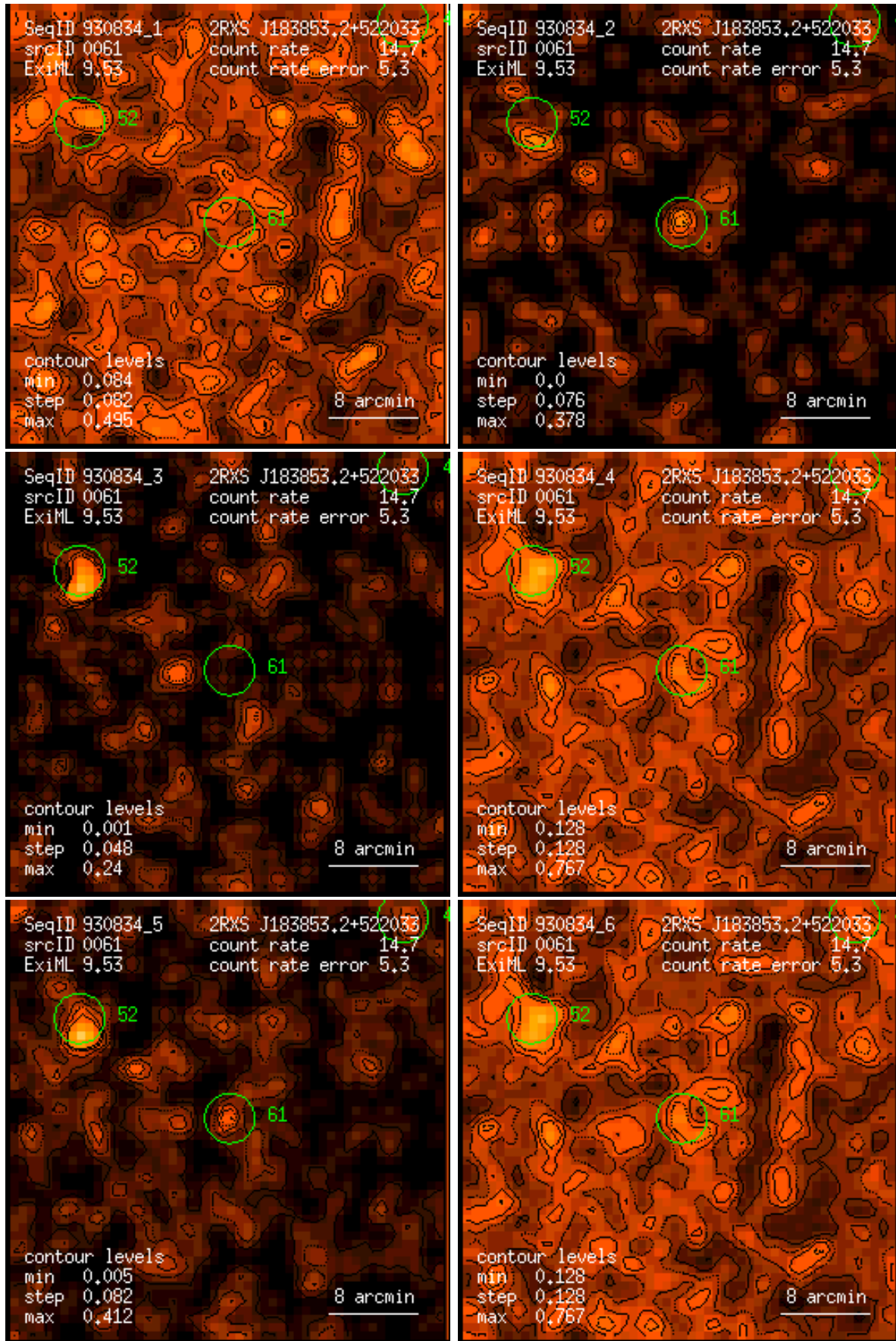
Figure 61: RASS 930834: detection 0061: band rate images, Gaussian filter: (1) PSPC channels 11 – 41, (2) 52 – 90, (3) 91 – 201, (4) 11 – 235, (5) 52 – 201, (6) 11 – 201. Broad band rates in counts/ks. Band rate contour levels in counts/ks/arcmin 2 .
