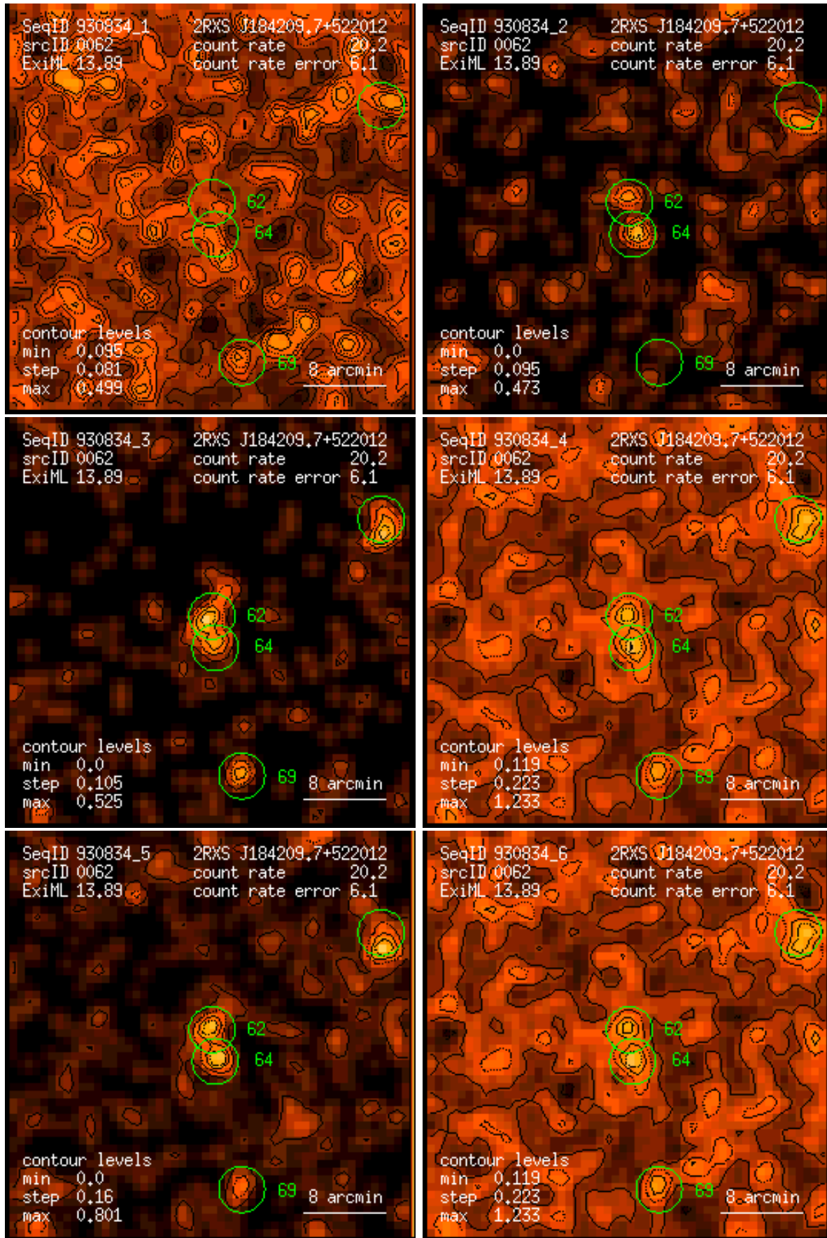
Figure 62: RASS 930834: detection 0062: band rate images, Gaussian filter: (1) PSPC channels 11 – 41, (2) 52 – 90, (3) 91 – 201, (4) 11 – 235, (5) 52 – 201, (6) 11 – 201. Broad band rates in counts/ks. Band rate contour levels in counts/ks/arcmin 2 .
