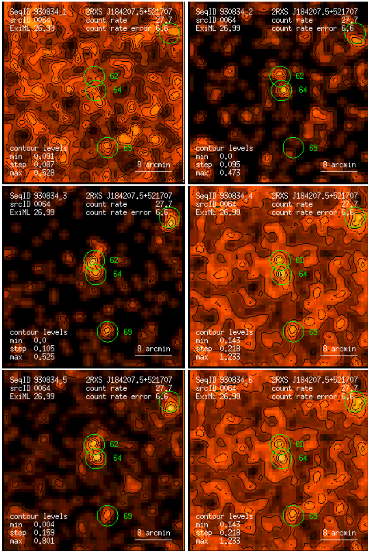
Figure 64: RASS 930834: detection 0064: band rate images, Gaussian filter: (1) PSPC channels 11 – 41, (2) 52 – 90, (3) 91 – 201, (4) 11 – 235, (5) 52 – 201, (6) 11 – 201. Broad band rates in counts/ks. Band rate contour levels in counts/ks/arcmin 2 .
