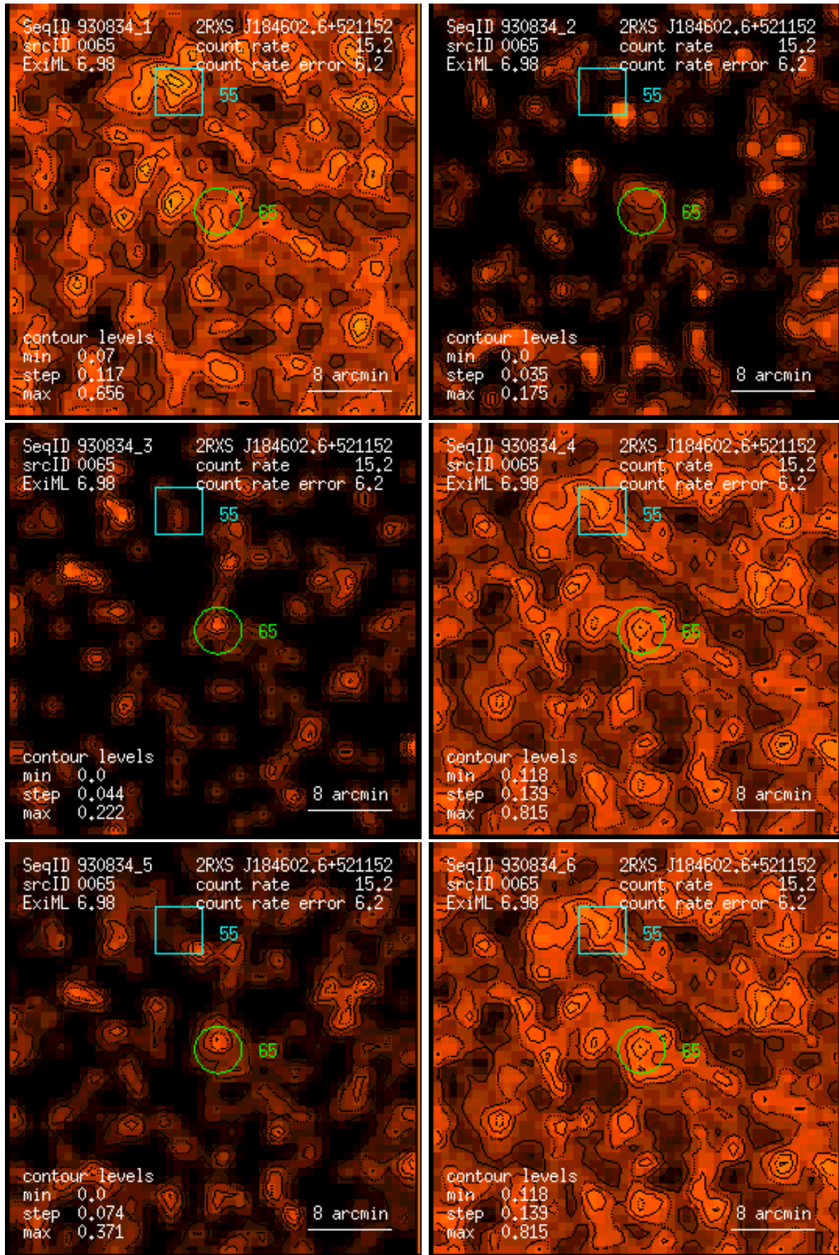
Figure 65: RASS 930834: detection 0065: band rate images, Gaussian filter: (1) PSPC channels 11 – 41, (2) 52 – 90, (3) 91 – 201, (4) 11 – 235, (5) 52 – 201, (6) 11 – 201. Broad band rates in counts/ks. Band rate contour levels in counts/ks/arcmin 2 .
