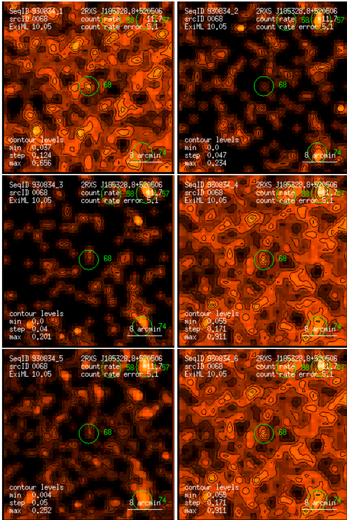
Figure 68: RASS 930834: detection 0068: band rate images, Gaussian filter: (1) PSPC channels 11 – 41, (2) 52 – 90, (3) 91 – 201, (4) 11 – 235, (5) 52 – 201, (6) 11 – 201. Broad band rates in counts/ks. Band rate contour levels in counts/ks/arcmin 2 .
