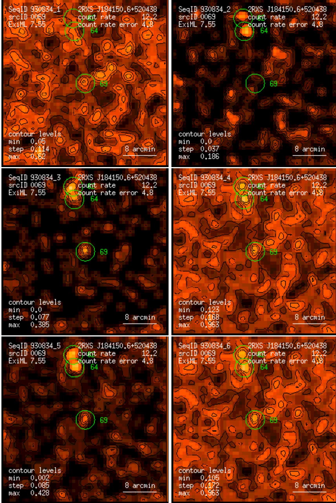
Figure 69: RASS 930834: detection 0069: band rate images, Gaussian filter: (1) PSPC channels 11 – 41, (2) 52 – 90, (3) 91 – 201, (4) 11 – 235, (5) 52 – 201, (6) 11 – 201. Broad band rates in counts/ks. Band rate contour levels in counts/ks/arcmin 2 .
