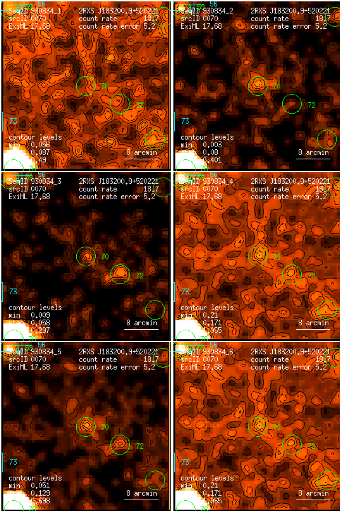
Figure 70: RASS 930834: detection 0070: band rate images, Gaussian filter: (1) PSPC channels 11 – 41, (2) 52 – 90, (3) 91 – 201, (4) 11 – 235, (5) 52 – 201, (6) 11 – 201. Broad band rates in counts/ks. Band rate contour levels in counts/ks/arcmin 2 .
