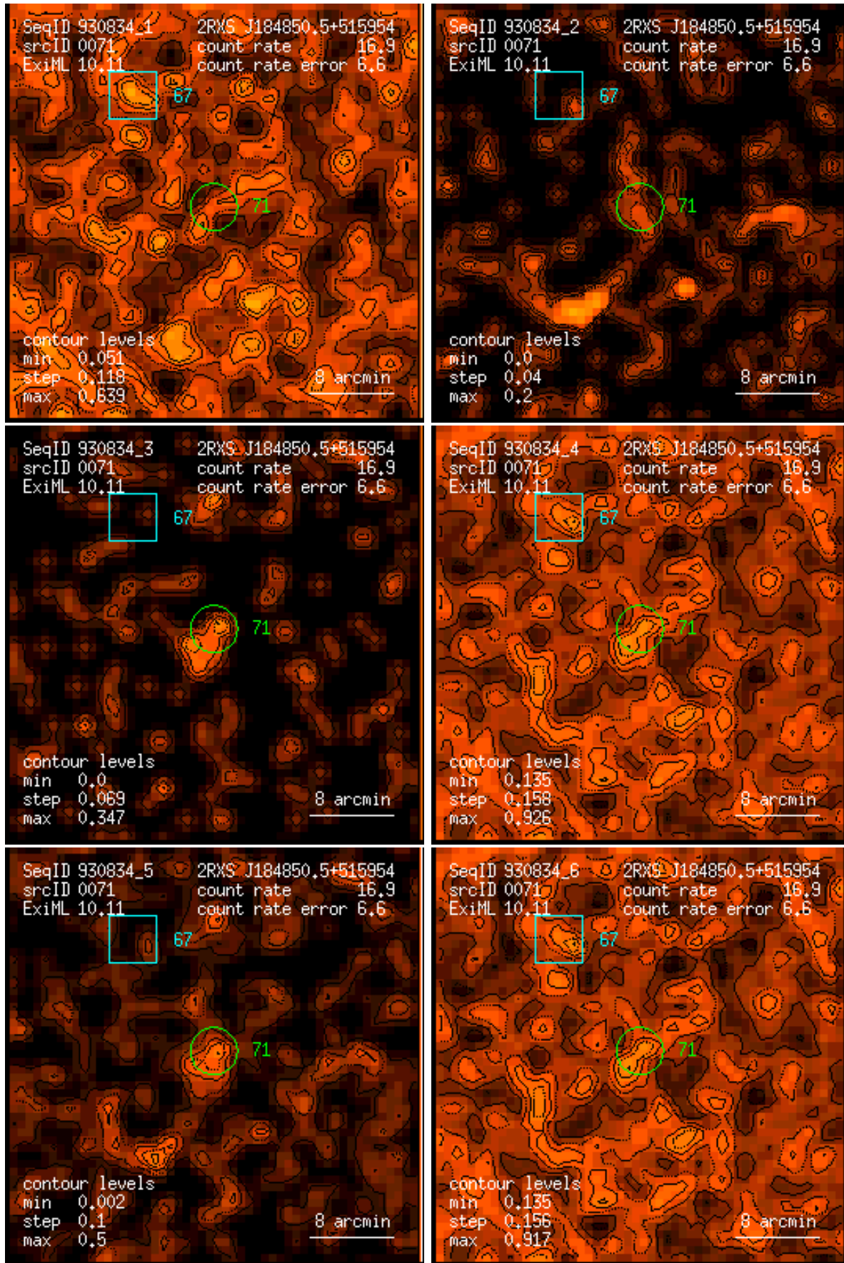
Figure 71: RASS 930834: detection 0071: band rate images, Gaussian filter: (1) PSPC channels 11 – 41, (2) 52 – 90, (3) 91 – 201, (4) 11 – 235, (5) 52 – 201, (6) 11 – 201. Broad band rates in counts/ks. Band rate contour levels in counts/ks/arcmin 2 .
