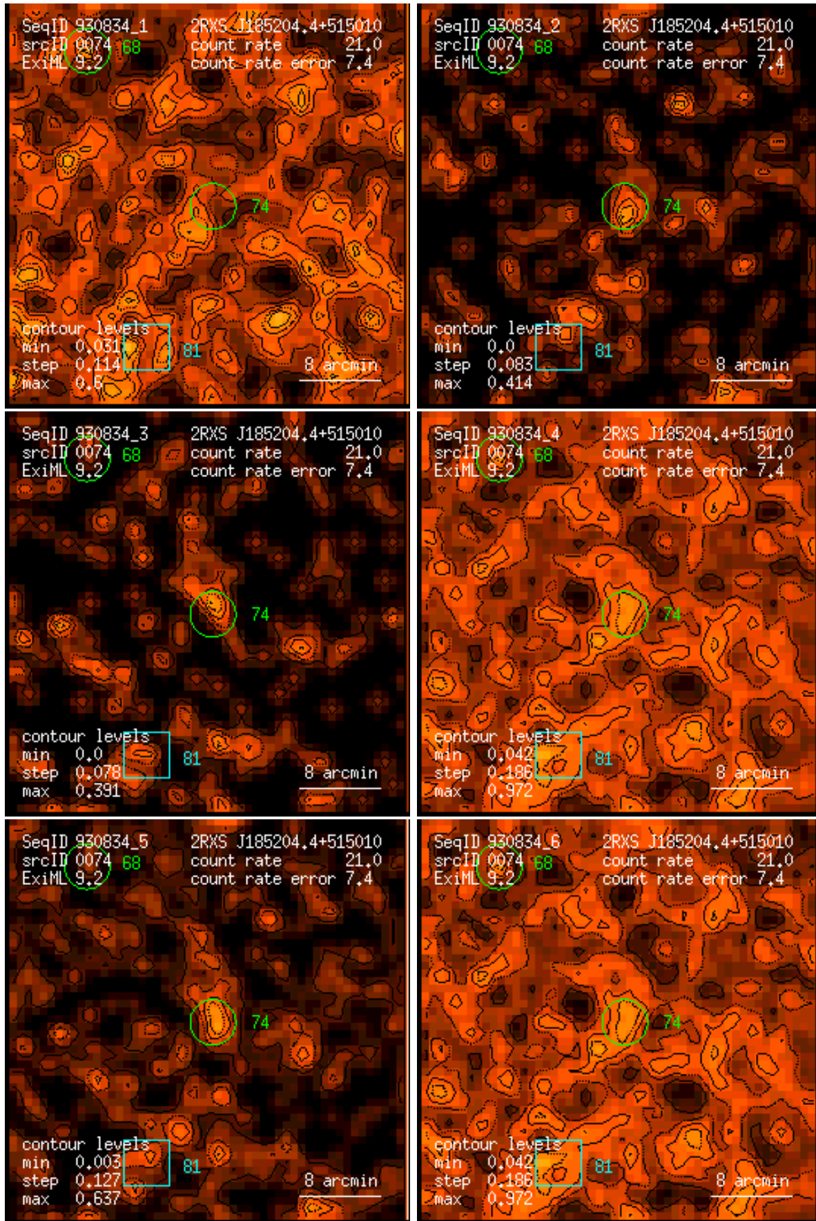
Figure 74: RASS 930834: detection 0074: band rate images, Gaussian filter: (1) PSPC channels 11 – 41, (2) 52 – 90, (3) 91 – 201, (4) 11 – 235, (5) 52 – 201, (6) 11 – 201. Broad band rates in counts/ks. Band rate contour levels in counts/ks/arcmin 2 .
