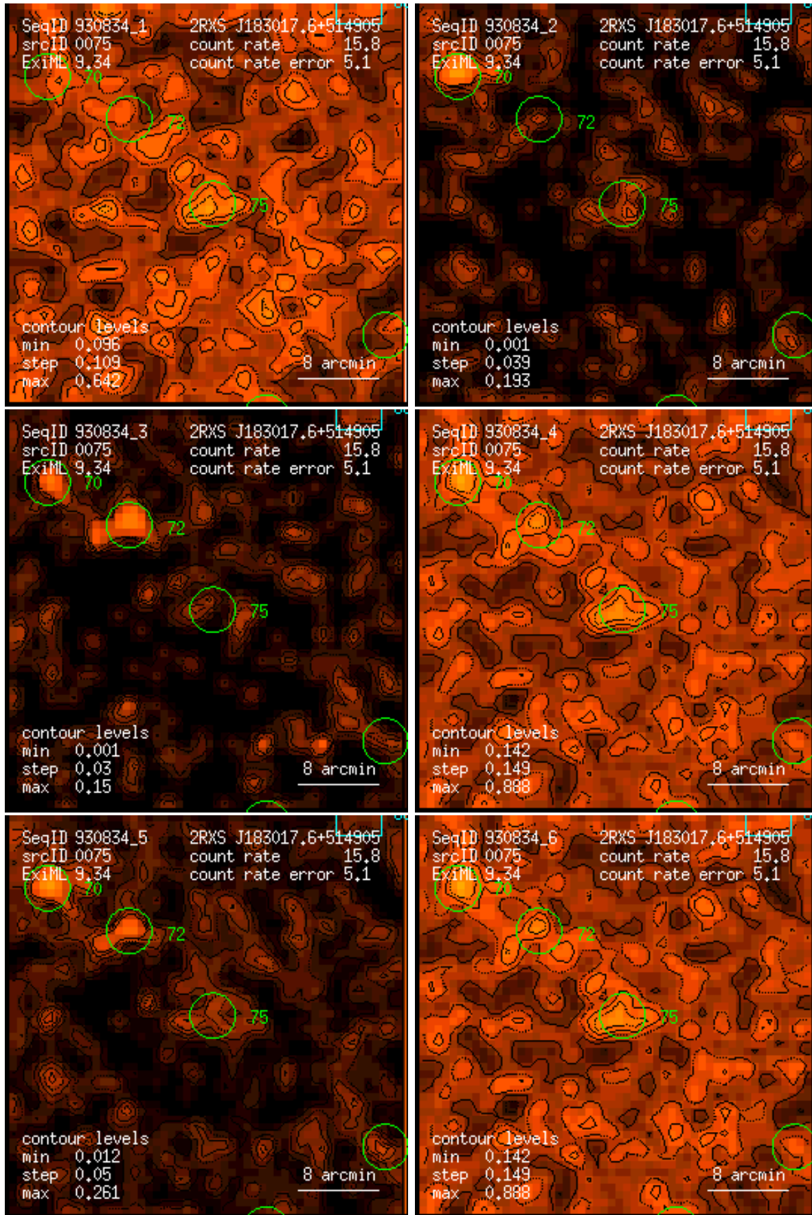
Figure 75: RASS 930834: detection 0075: band rate images, Gaussian filter: (1) PSPC channels 11 – 41, (2) 52 – 90, (3) 91 – 201, (4) 11 – 235, (5) 52 – 201, (6) 11 – 201. Broad band rates in counts/ks. Band rate contour levels in counts/ks/arcmin 2 .
