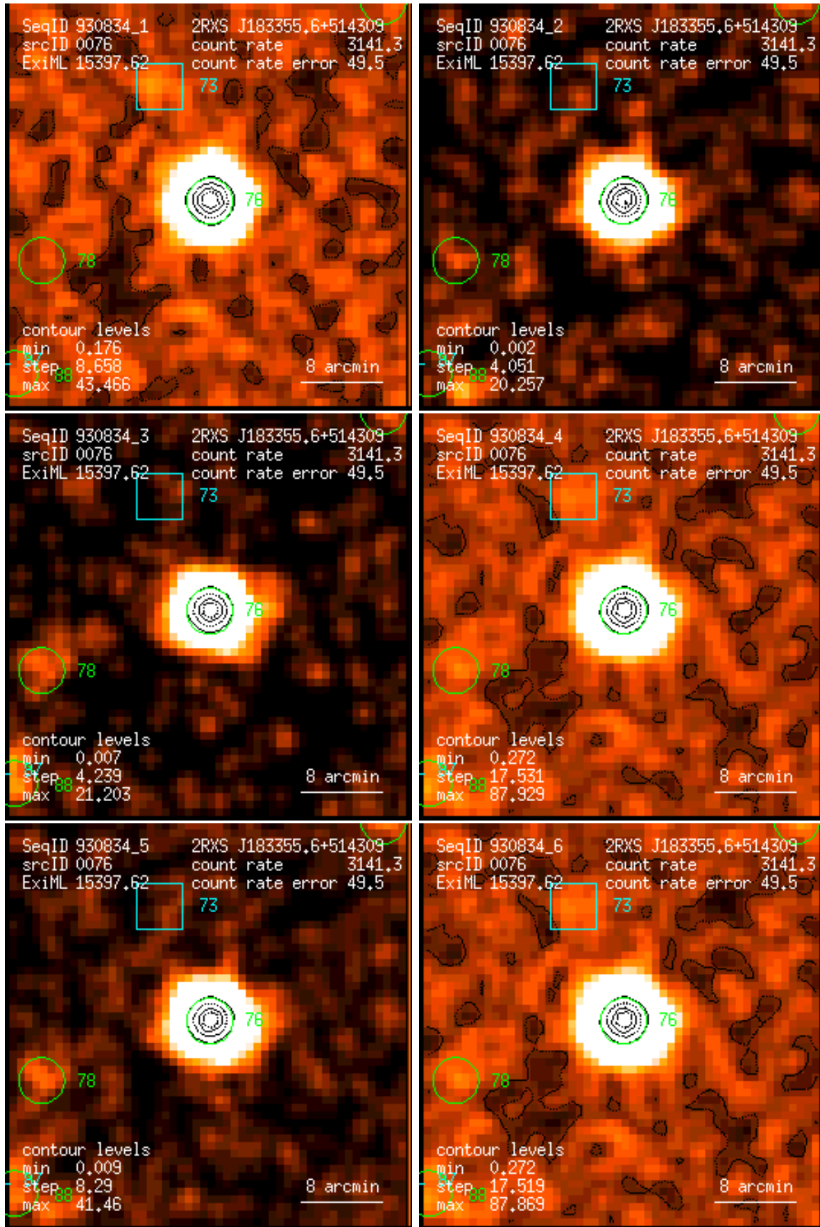
Figure 76: RASS 930834: detection 0076: band rate images, Gaussian filter: (1) PSPC channels 11 – 41, (2) 52 – 90, (3) 91 – 201, (4) 11 – 235, (5) 52 – 201, (6) 11 – 201. Broad band rates in counts/ks. Band rate contour levels in counts/ks/arcmin 2 .
